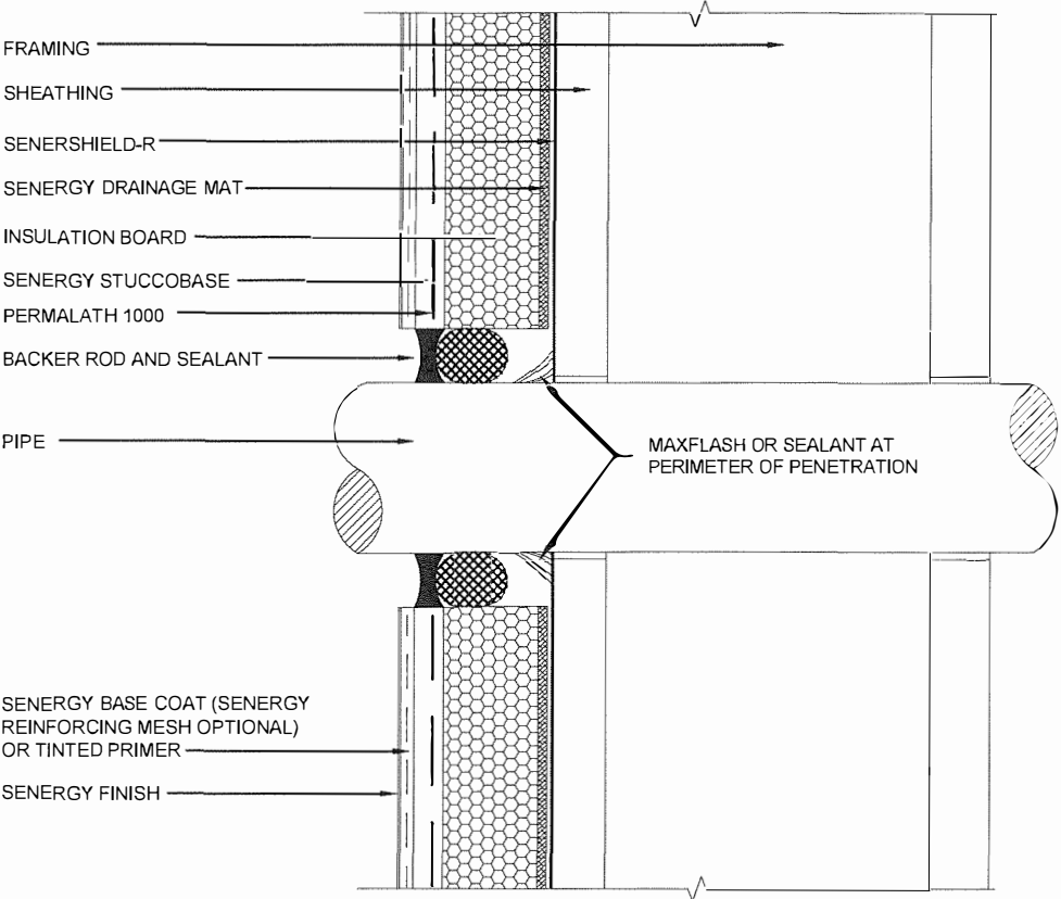
PIPE PENETRATION
