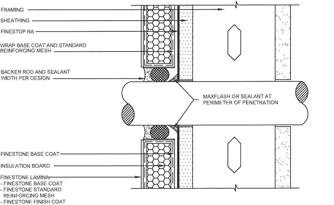
PIPE PENETRATION
