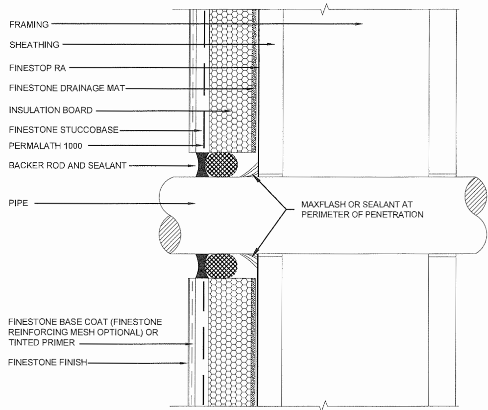
PIPE PENETRATION
