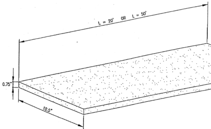
Roof Saver Attic Vent Media
