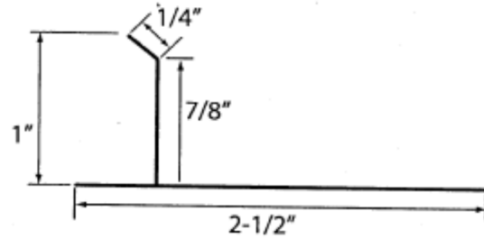
Deflector
