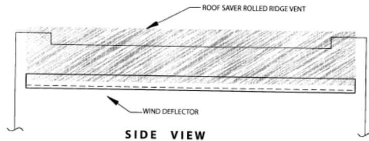
Installed Roof Saver Attic Vent System
