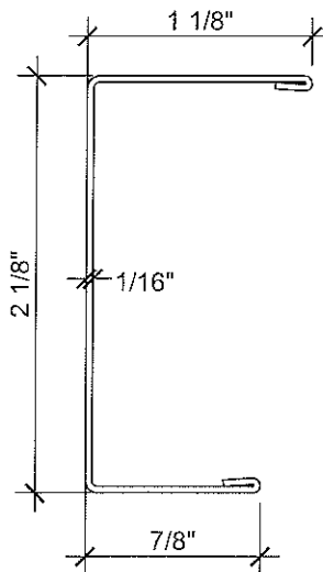
U 2- 3 / 32 CHANNEL WALL MOLDING (3003 H14)
