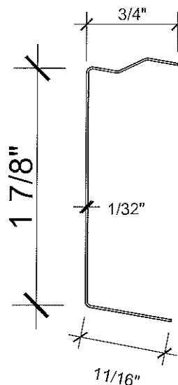
U 2- 3 / 32 HOLD- DOWN CLIP
