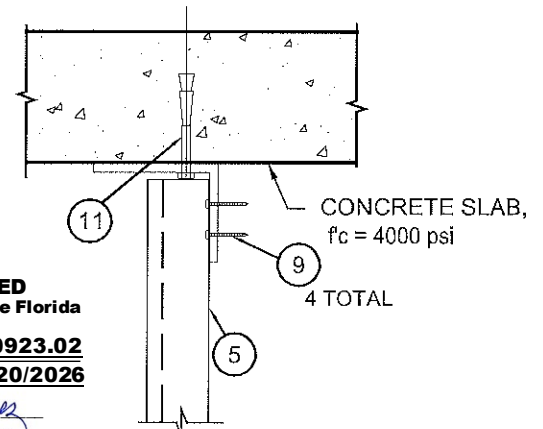
DETAIL 9
