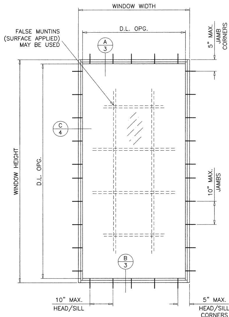
TYPICAL ELEVATION
