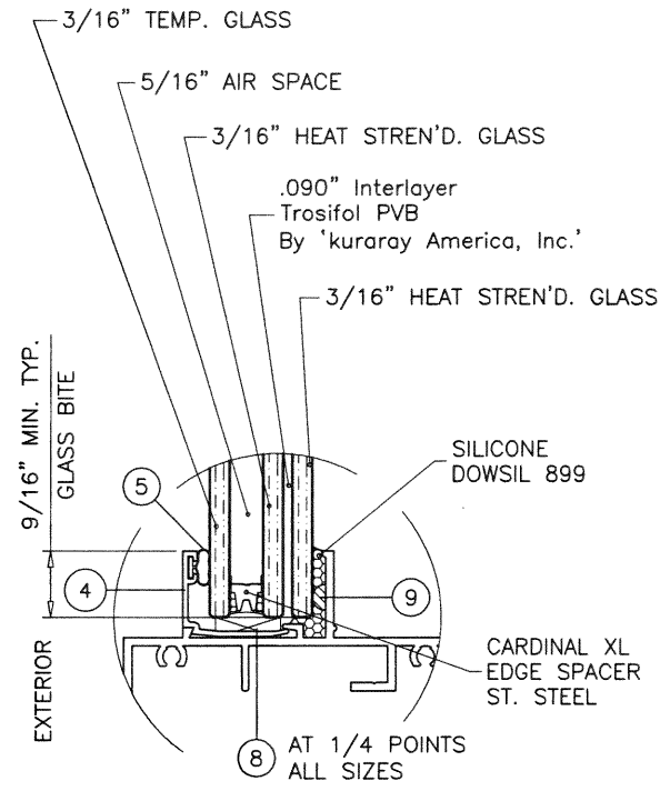
GLASS TYPE 'G2i' 15/16" OVERALL INSUL. LAM. GLASS
