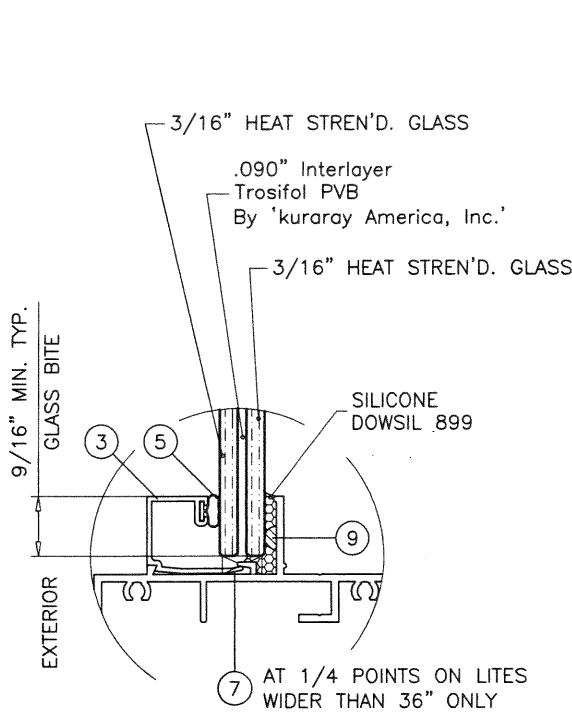
GLASS TYPE 'G2' 7/16" OVERALL LAM. GLASS
