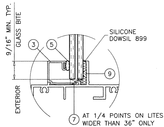
GLASS TYPE 'G1' 7/16" OVERALL LAM. GLASS
