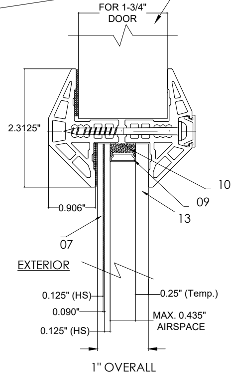
GLAZING TYPE B INSULATED, LAMINATED GLASS WITH MELTED GLASS
