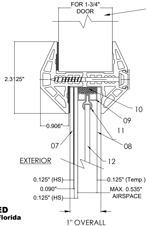
GLAZING TYPE A INSULATED, LAMINATED GLASS WITH DECORATIVE GLASS
