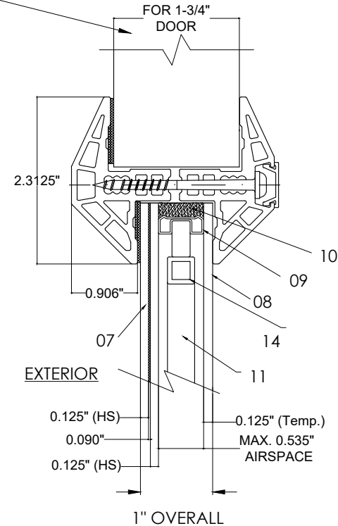
GLAZING TYPE C INSULATED, LAMINATED GLASS WITH WROUGHT IRON
