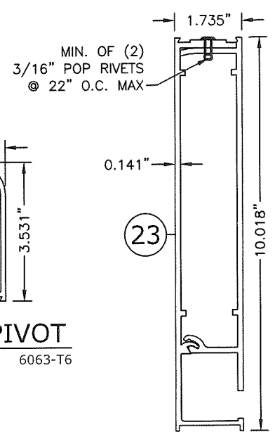
(SERIES 2000) BOTTOM RAIL, O N.T.S. 2-PIECE 6063-T6
