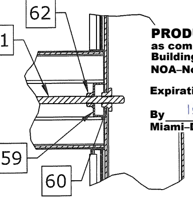
M MUNTIN DETAIL NTS SERIES 2000/3000
