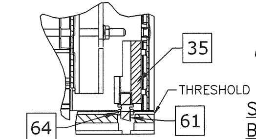
B SO PIVOT BOTTOM NTS SERIES 3000
