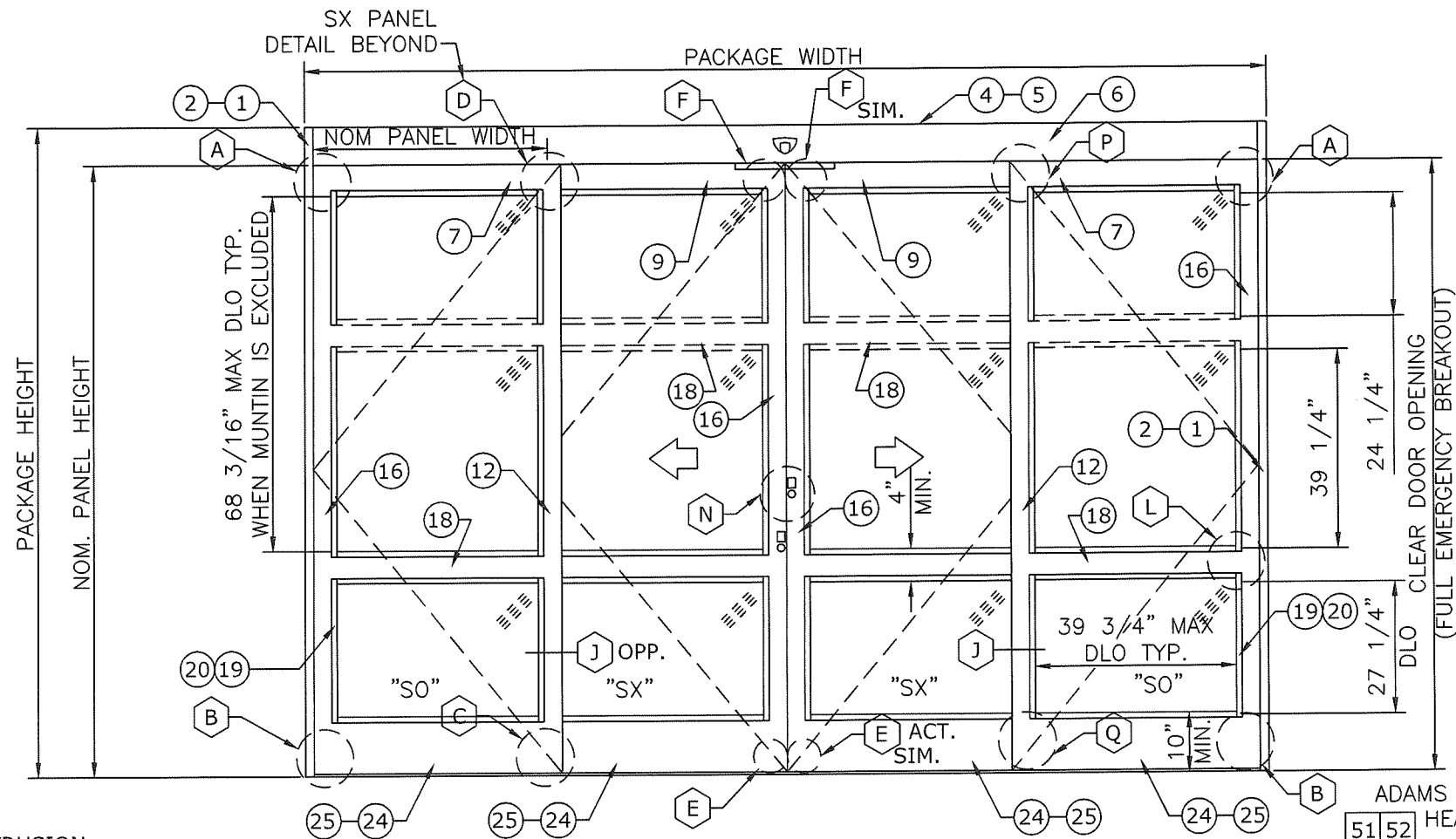
EXTERIOR ELEVATION
