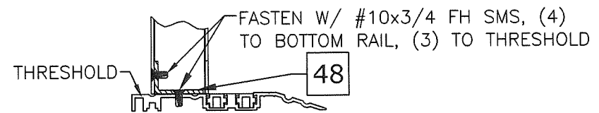
I O-PANEL BRACKET NTS SERIES 2000
