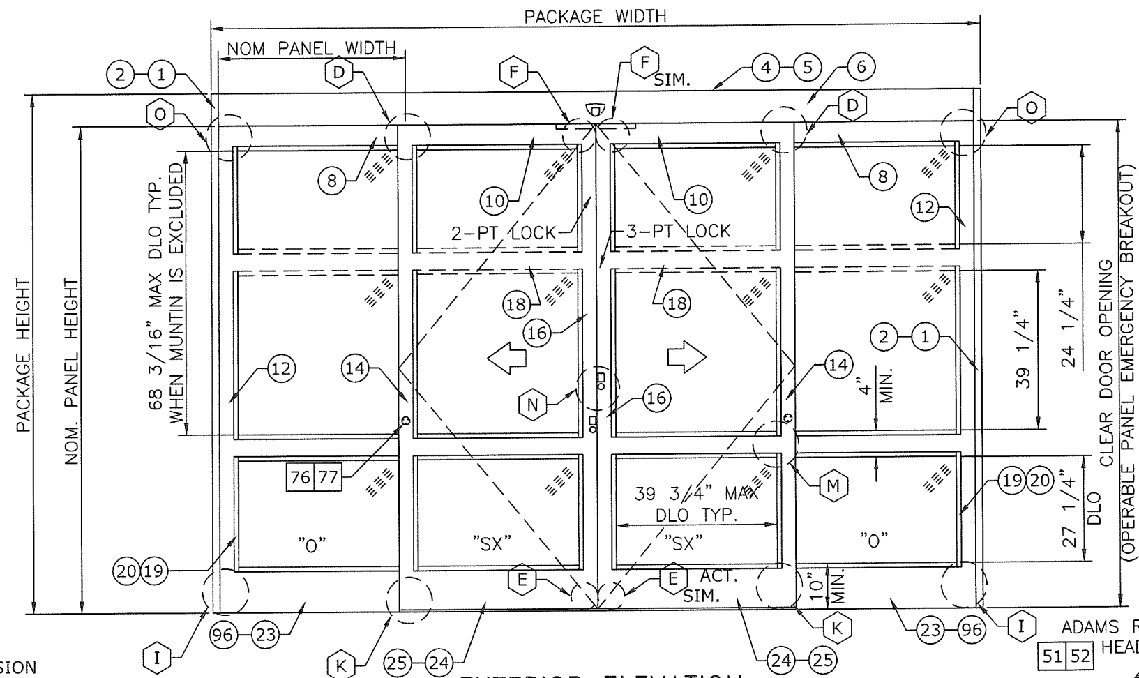
EXTERIOR ELEVATION
