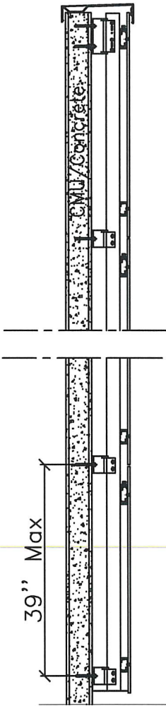
A-A Vertical Section
