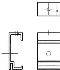
①B Primary C-clamp
