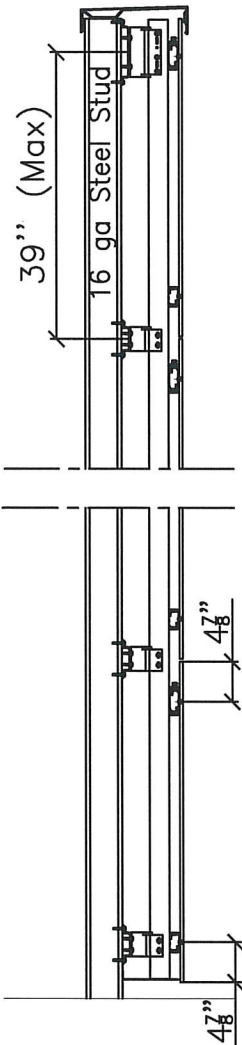
A-A Vertical Section
