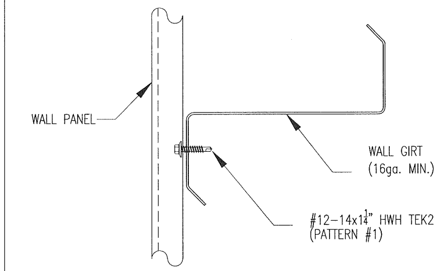
WALL DETAIL @ INTERMEDIATE GIRT
