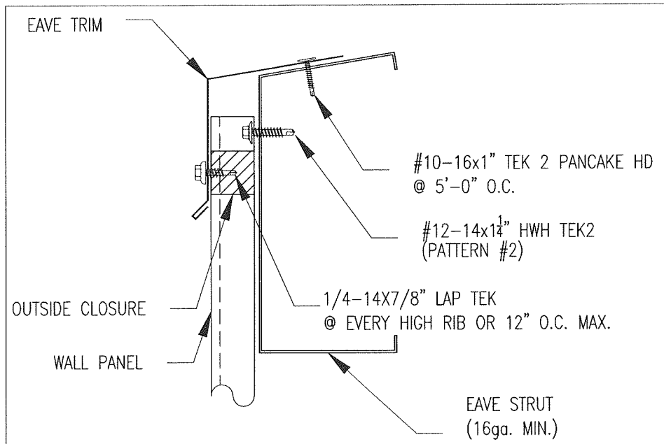
WALL DETAIL @ EAVE
