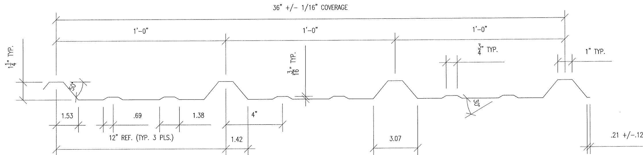
TREMLOCK R STEEL WALL PANEL PROFILE
