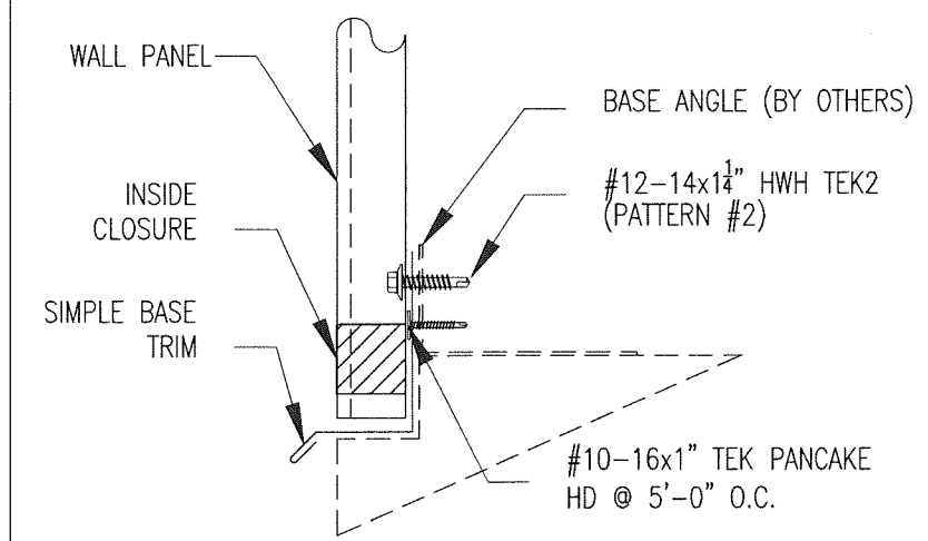
WALL DETAIL @ BASE
