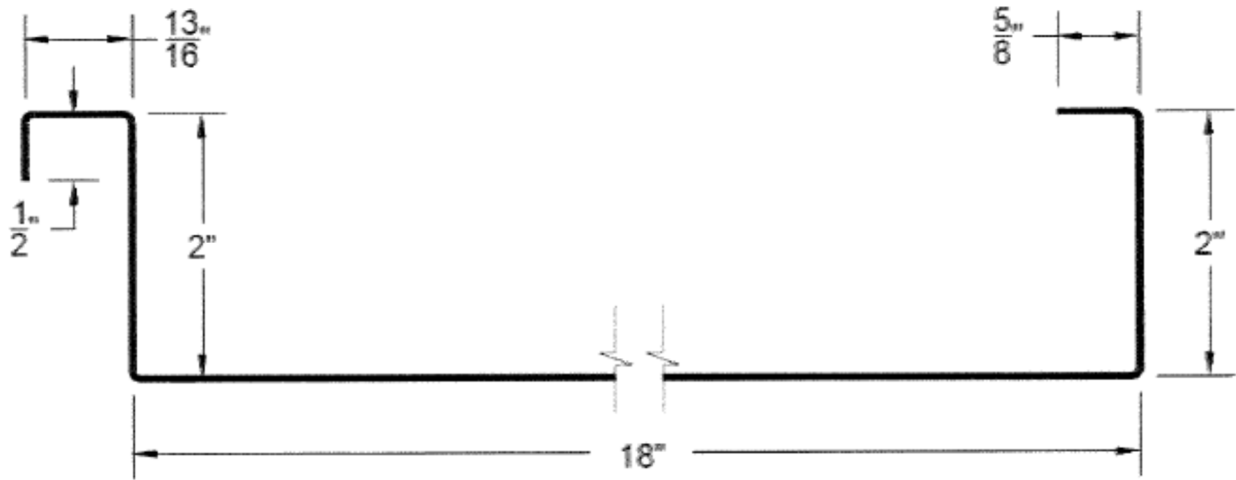
DCM 200 S – 0.032" ALUMINUM PANEL
