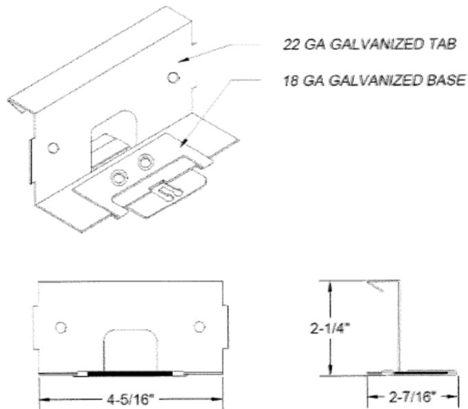
TWO-PIECE CLIP
