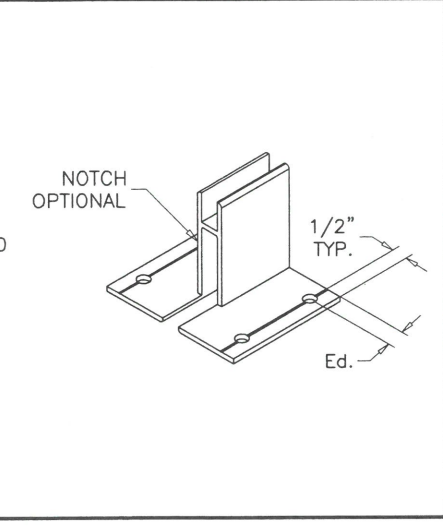
53 FLUSH FRAME ADAPTER
