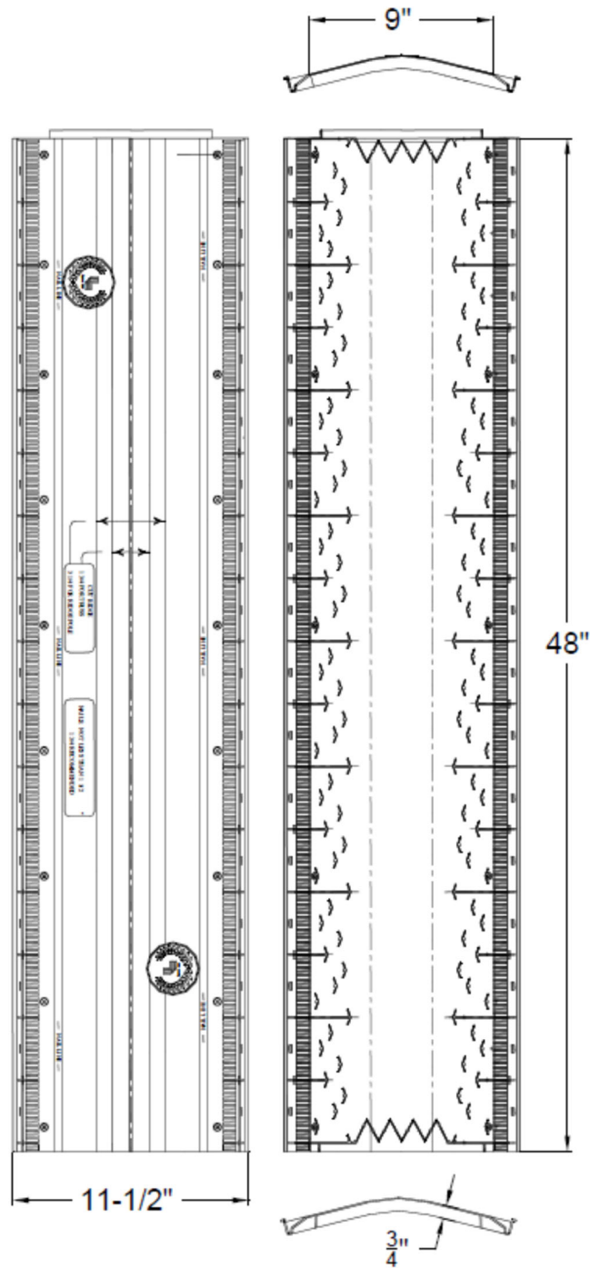
TopShield® Lo-OmniRidge TSLOR9-4 Ridge Vent
