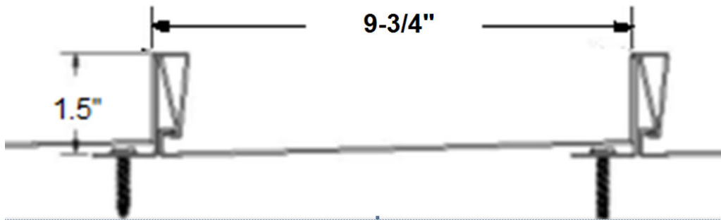
UC-4 METAL ROOF PANEL
