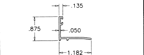
2A GLASS STOP (INSUL. LAM. GLASS)
