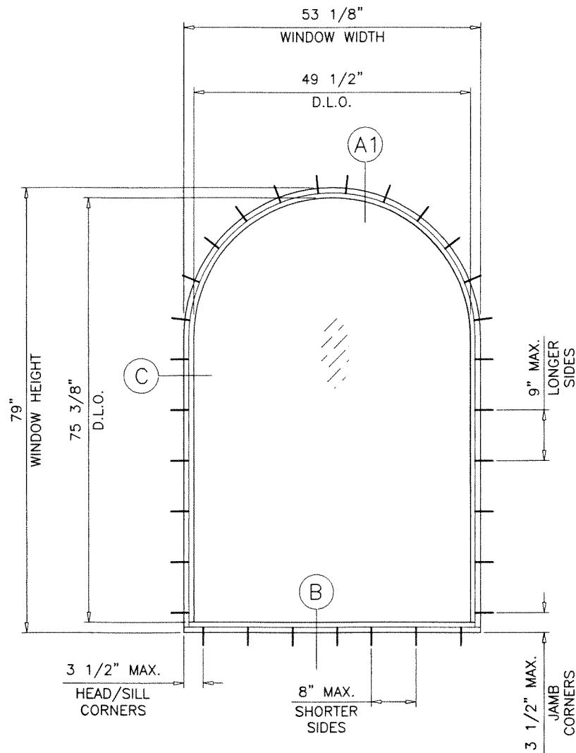
TYPICAL ELEVATIONS
