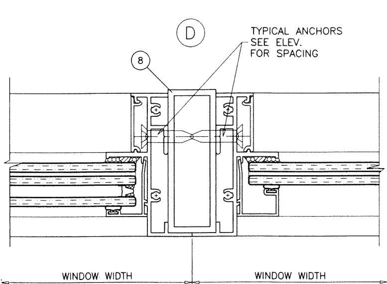
MULLION TYPE '1'
