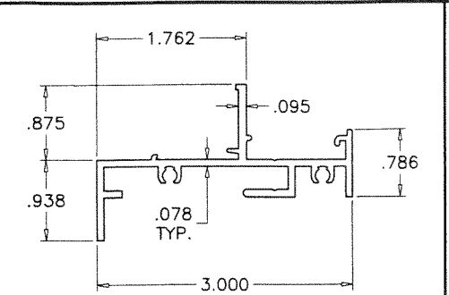
1 FRAME HEAD/SILL/JAMB
