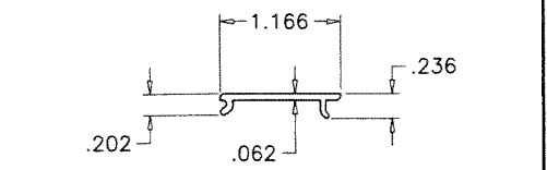
3 FRAME COVER
