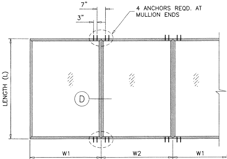
TYPICAL ELEVATIONS SIDE BY SIDE WINDOWS SIDE BY SIDE APPLIES TO TWO OR MORE WINDOWS
