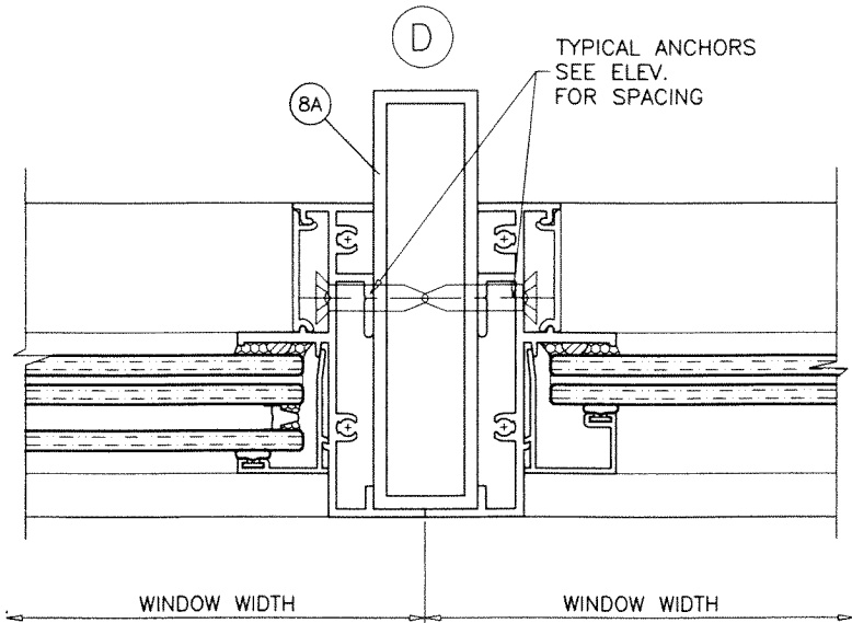
MULLION TYPE '2'
