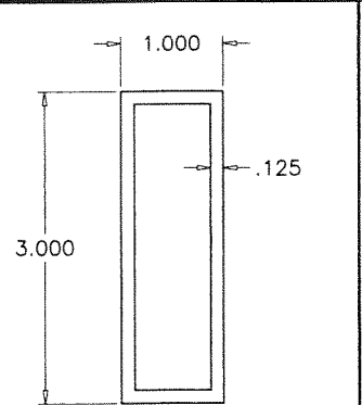
8 TUBE MULLION
