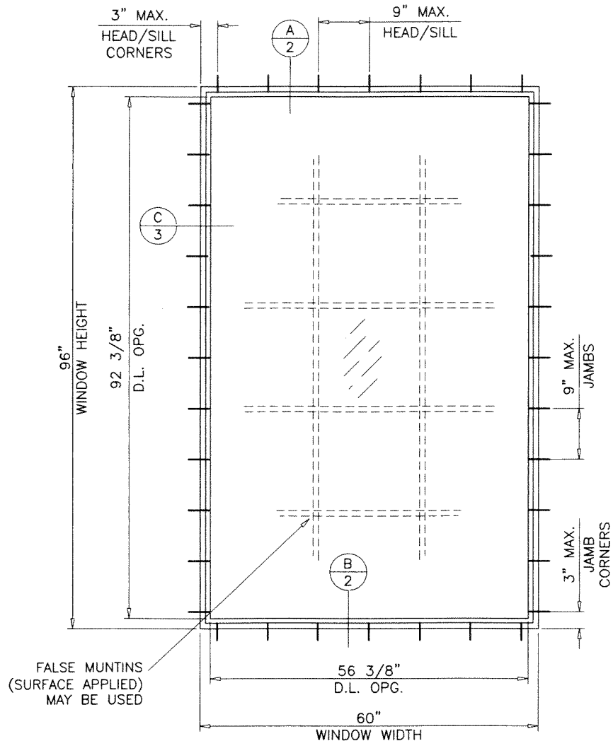
TYPICAL ELEVATIONS
