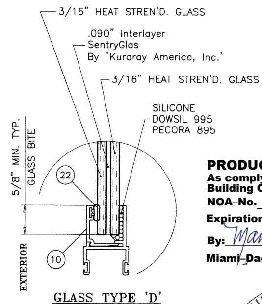
GLAZING DETAIL FIX. LITE
