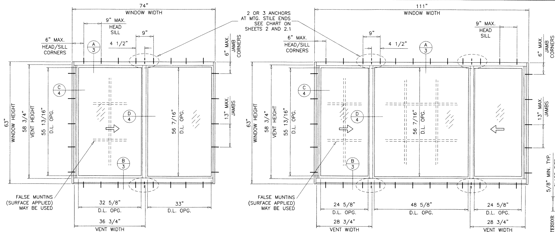
TYPICAL ELEVATIONS
