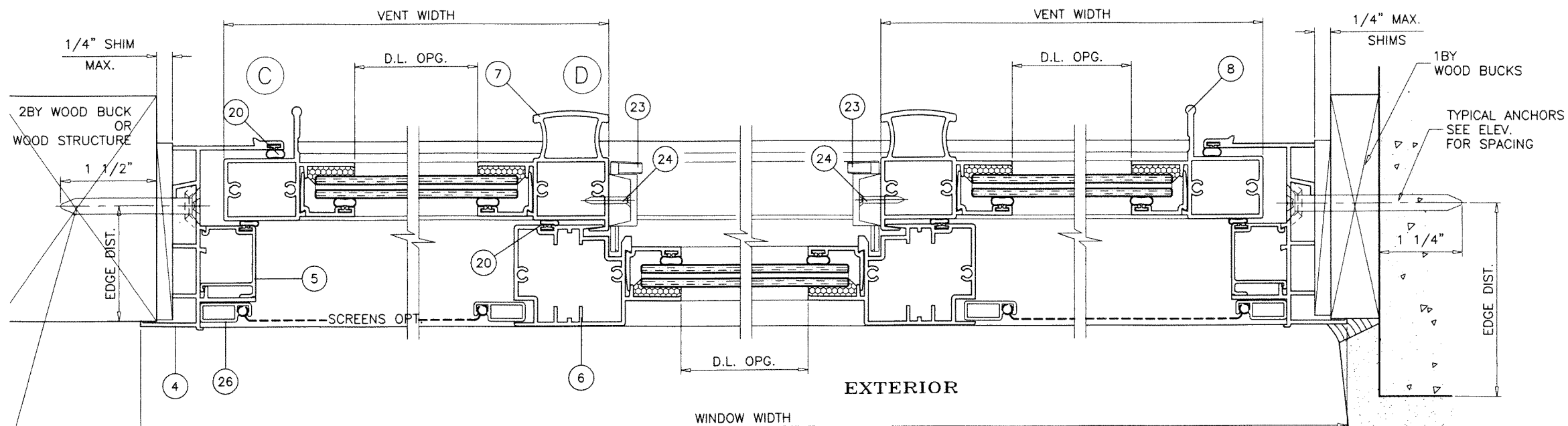
XOX LAYOUT
