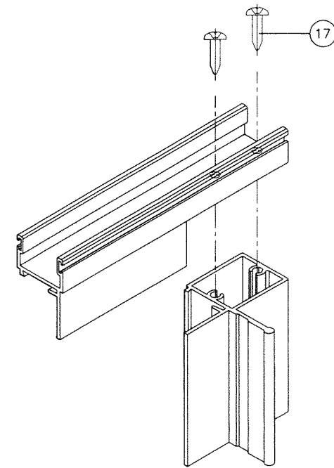
VENT TOP/BOTTOM CORNERS
