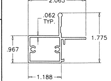
1 FRAME HEAD
