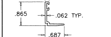
10 GLAZING BEAD
