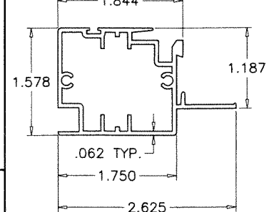
3 SILL TRACK
