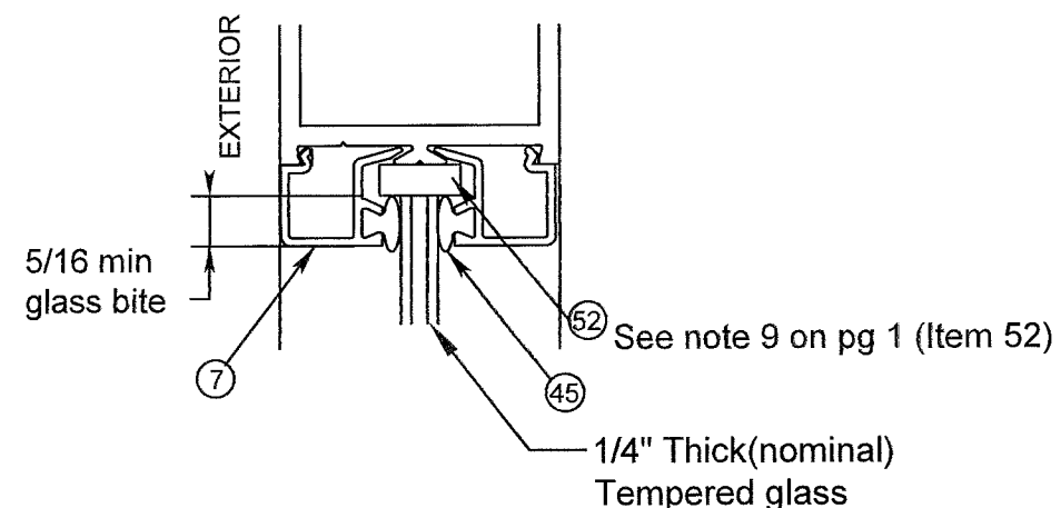
GLAZING DETAIL
