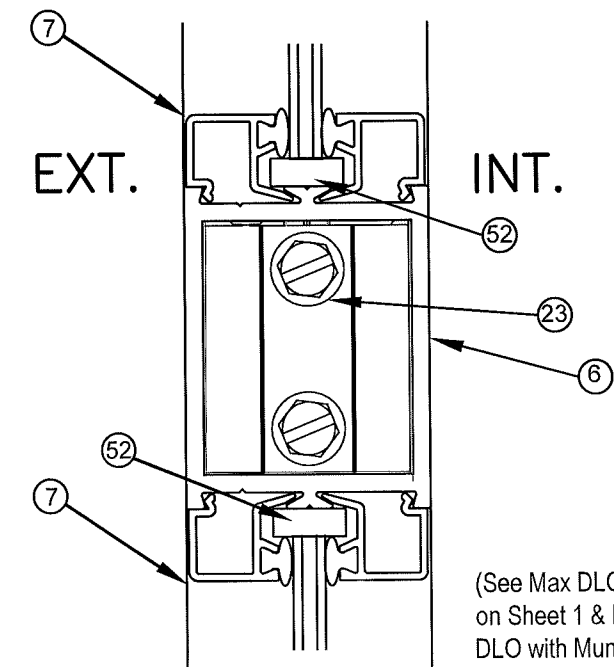
MUNTIN OPTION
