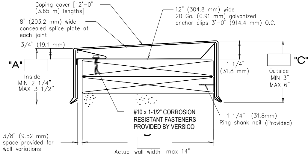
VERSiTRIM 200 COPING (14" WIDE)
