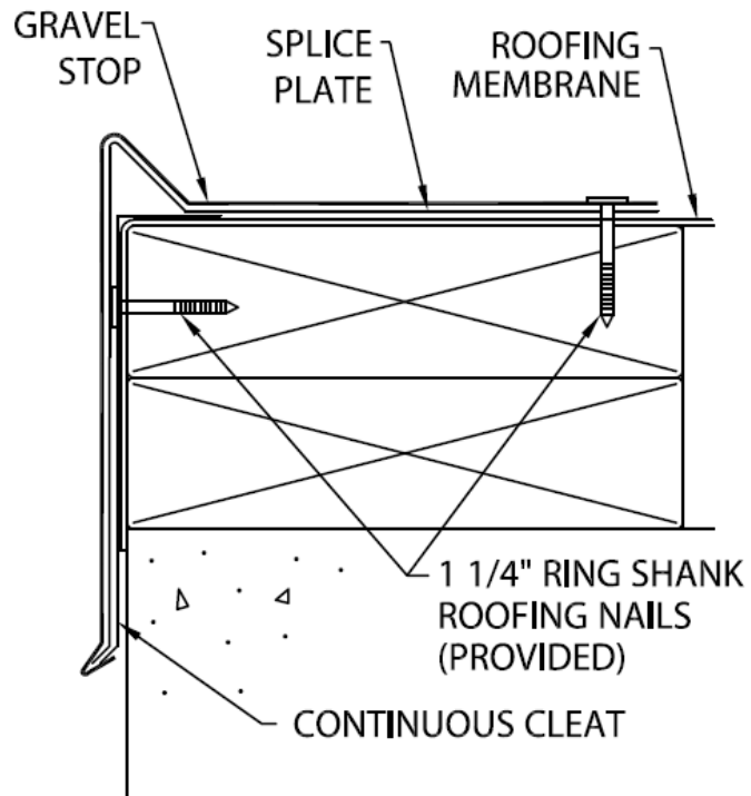
VERSiTRIM 200 GRAVEL STOP
