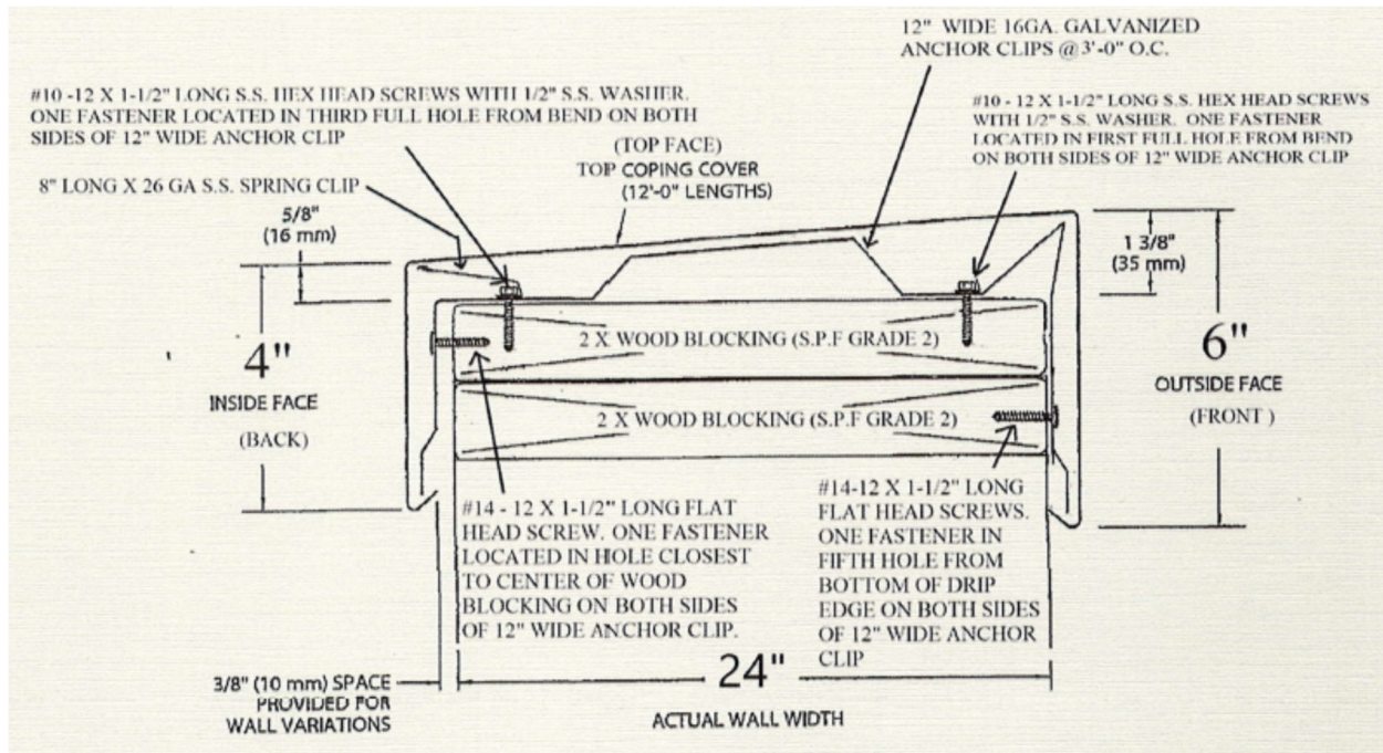
VERSiTRIM 200 GOLD COPING
