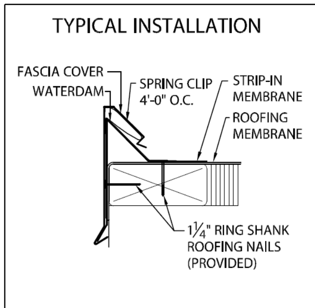
VERSiTRIM SYSTEM 200 FASCIA, CRIMP-ON OR SNAP-ON
