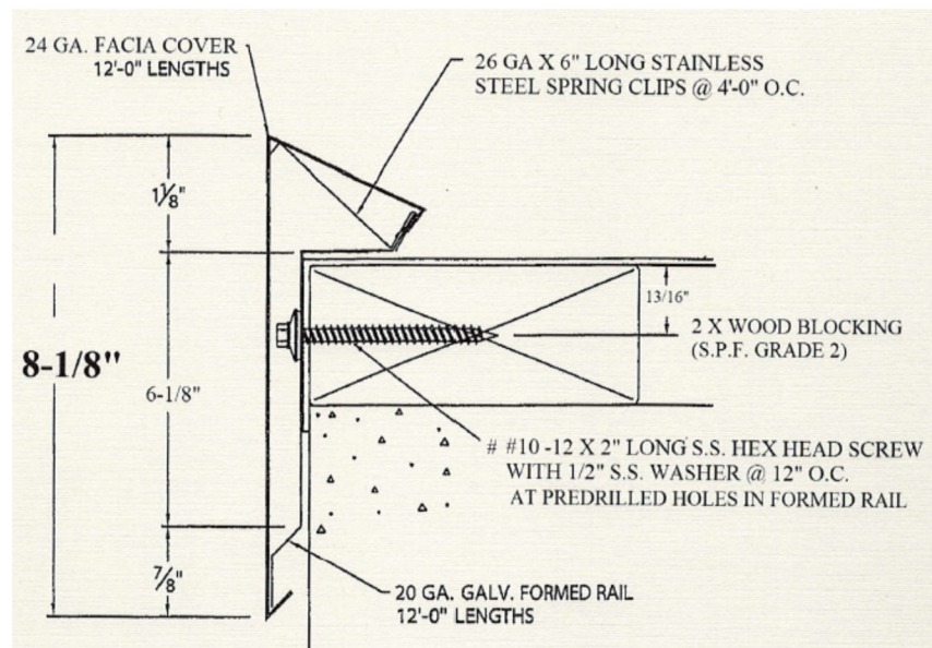
VERSiTRIM ONE FASCIA
