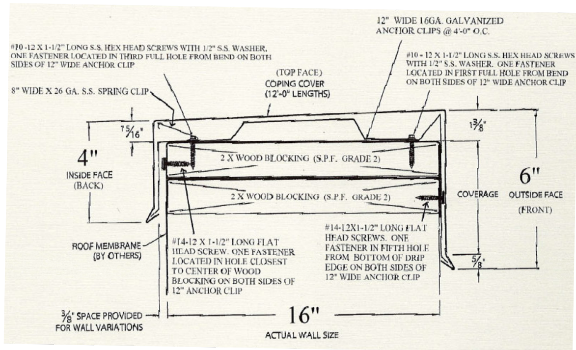
VERSiTRIM 200 COPING (16" WIDE)
