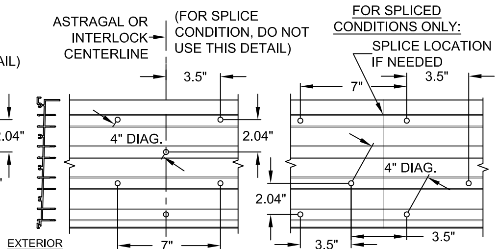
4-TRACK FRAME HEAD/SILL @ ASTRAGAL OR INTERLOCK (USE WHERE 6 CLUSTER ANCHORS ARE REQUIRED, "C6") WITH & WITHOUT SPLICE CONDITION
