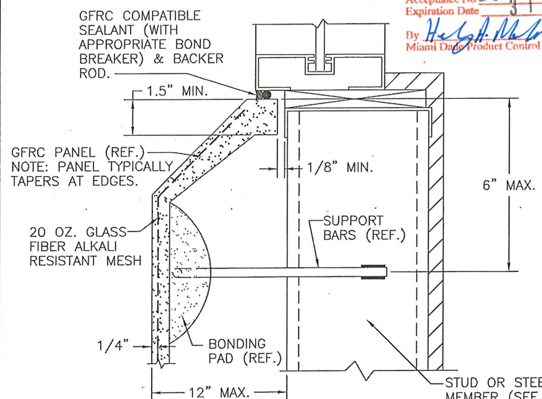
MISCELLANEOUS DETAIL
