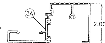
HI-RISE SILL
