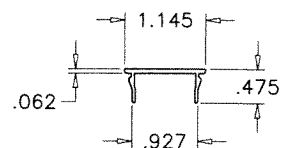
⑭ SILL COVER
