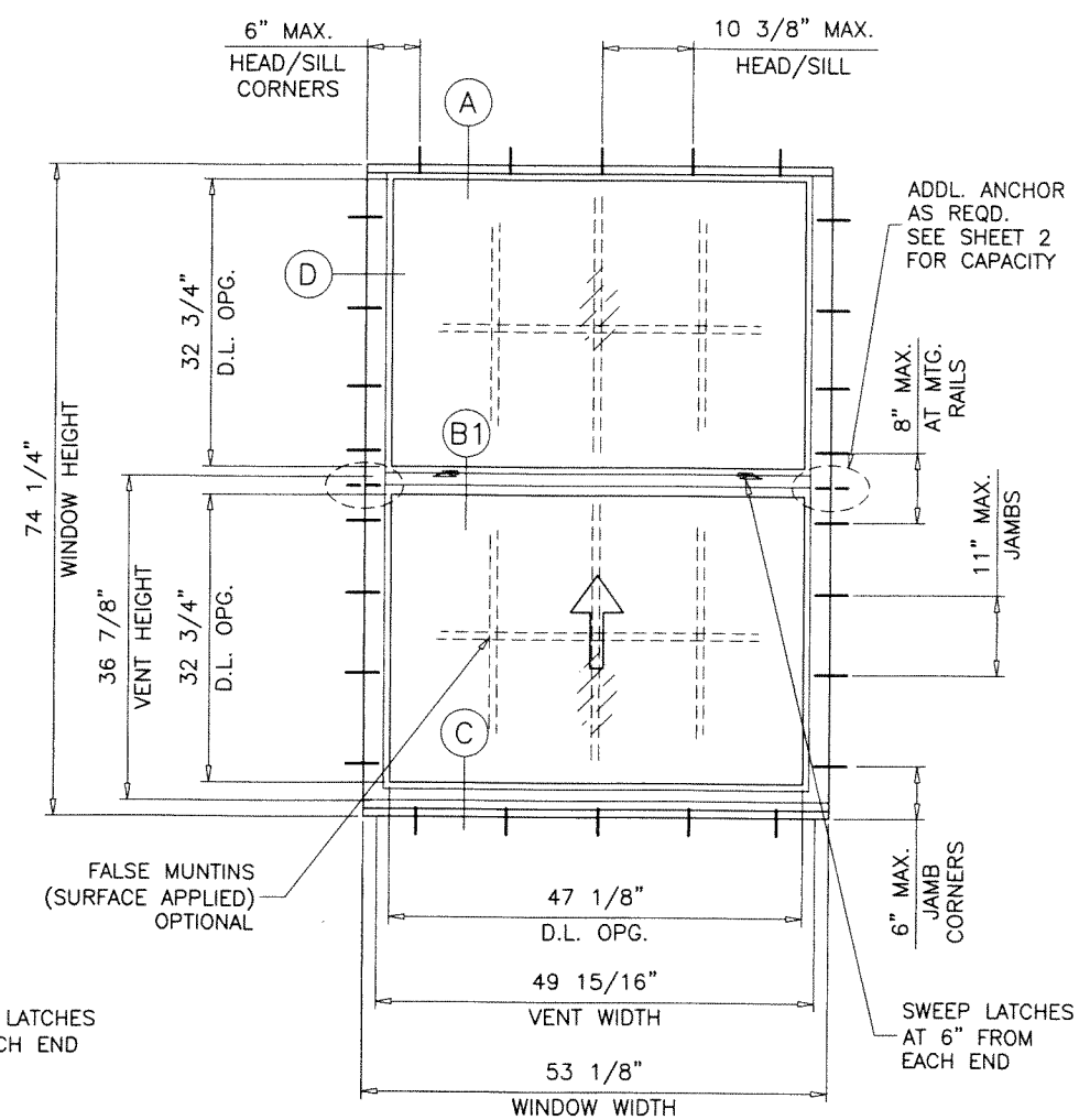
TYPICAL ELEVATION
