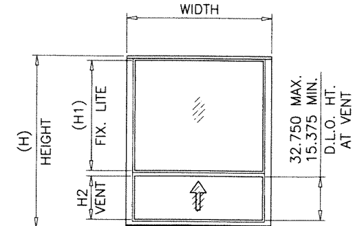
UNEQUAL LITES (ORIEL TYPE)
