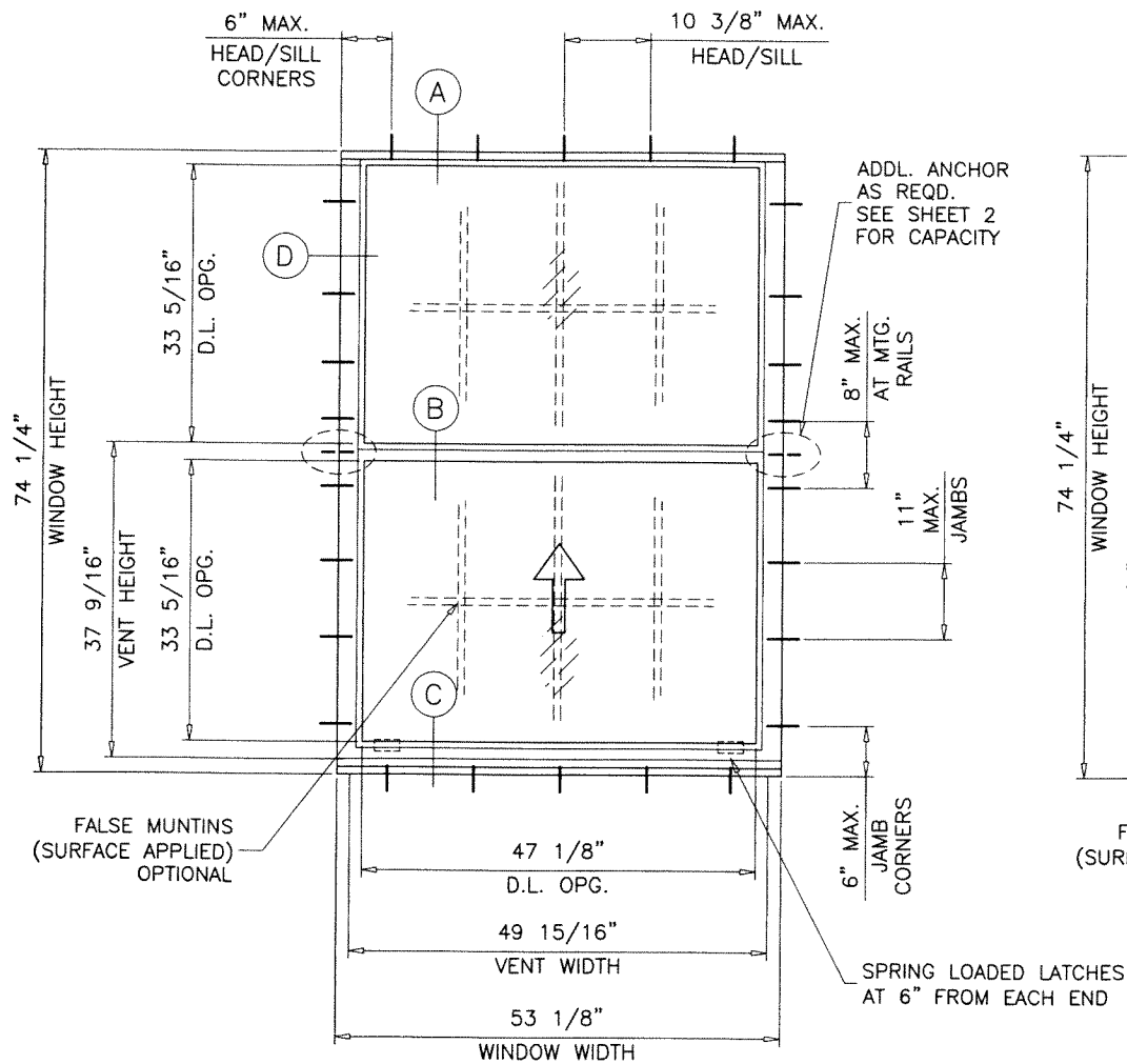
TYPICAL ELEVATION
