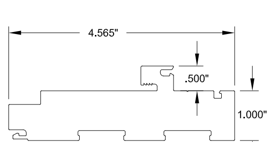
1 FRAME HEAD & JAMB #20000, Rigid Cellular PVC
