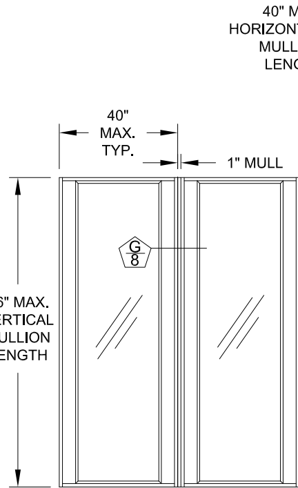
O|O (MAXIMUM OF 2 MULLED SIDELITES) (WIDE STILES AND NARROW RAILS SHOWN ON SIDELITES)
