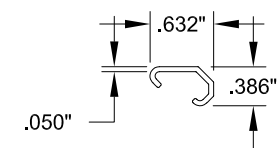
20 SINGLE DOOR ASTRAGAL COVER #20012, Rigid PVC
