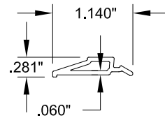
14 BEVELED BEAD #20005, Rigid PVC
