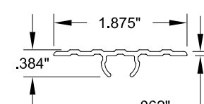
22 THRESHOLD COVER #20057, 6063-T5
