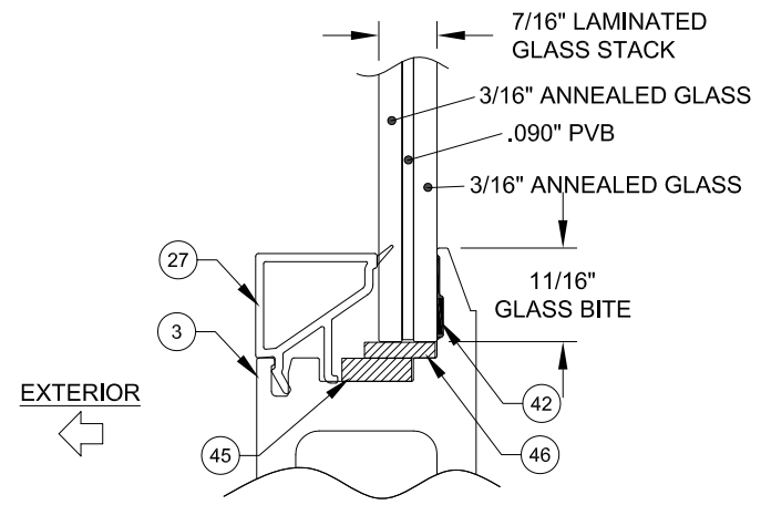
GLASS TYPE 7 USED IN DOOR, (SHOWN) & SIDELITE/TRANSOM
