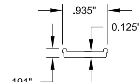
23 ANCHOR PLATE #19031, 6063-T6
