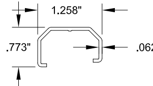
19 ACTIVE ASTRAGAL COVER #20011, Rigid PVC
