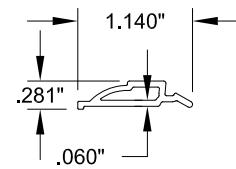
15 OGEE BEAD #20006, Rigid PVC
