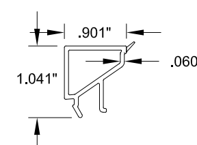
27 7/16\" SQUARE BEAD #20047, Rigid PVC
