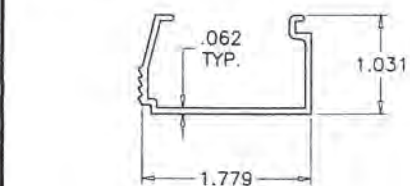
2 GLAZING STOP
