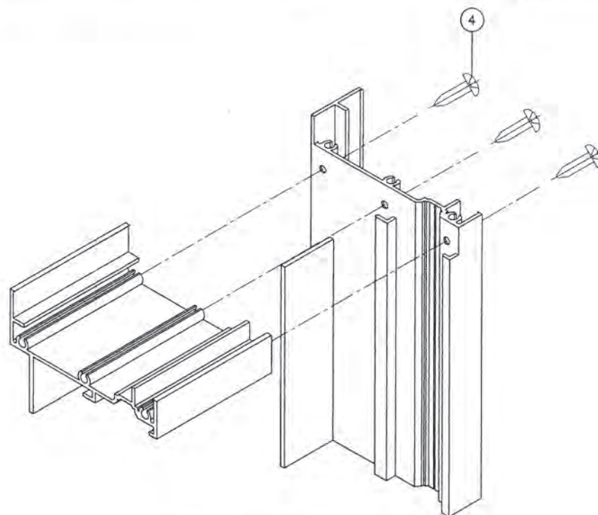
FRAME CORNERS
