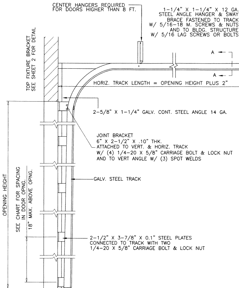
DOOR TRACK AS VIEWED FROM CENTER OF OPENING
