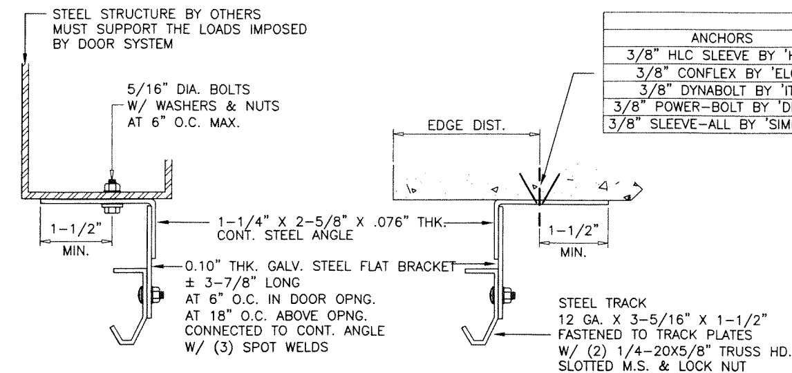
TRACK INSTALLATION
