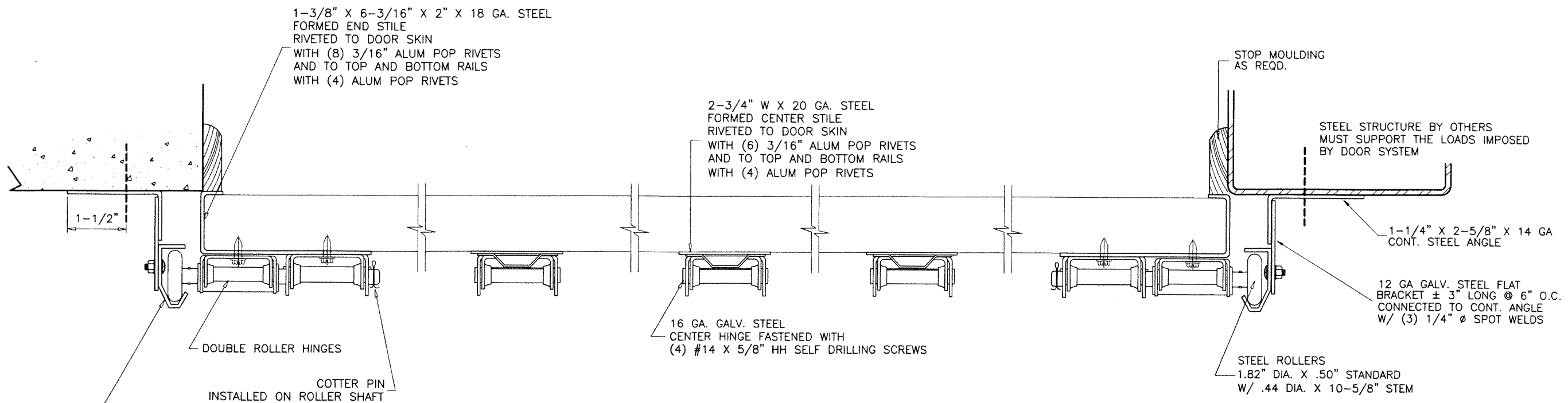
SECTION B-B
