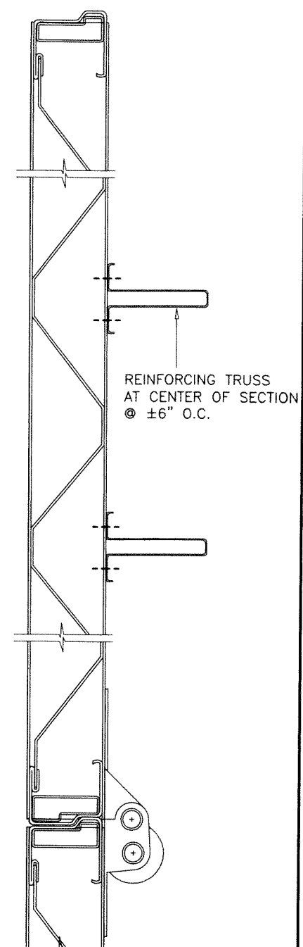
TOP SECTION AND ALL INTERMEDIATE SECTIONS REINFORCING
