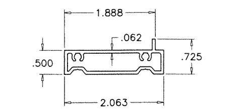
(E3) FLUSH FRAME ADAPTER
