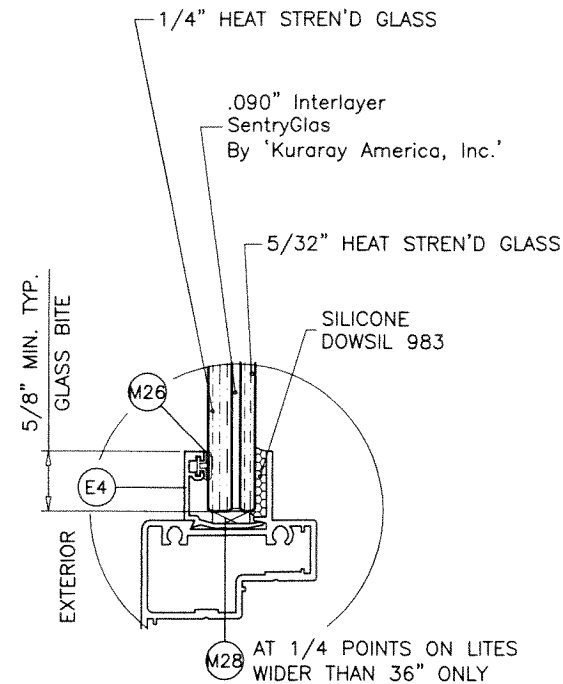
GLAZING DETAIL
