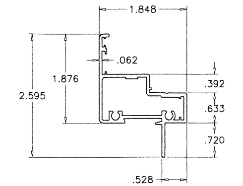
(E2) VENT
