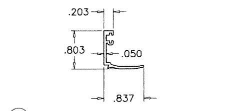
(E4) GLAZING STOP (LAM. GLASS)
