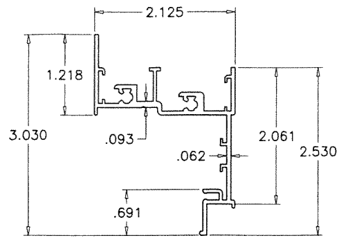
(E1) FRAME
