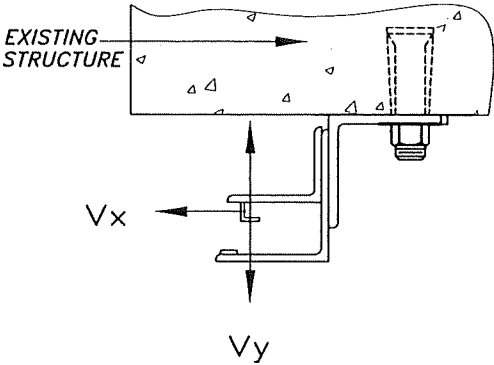
LOAD DIAGRAM
