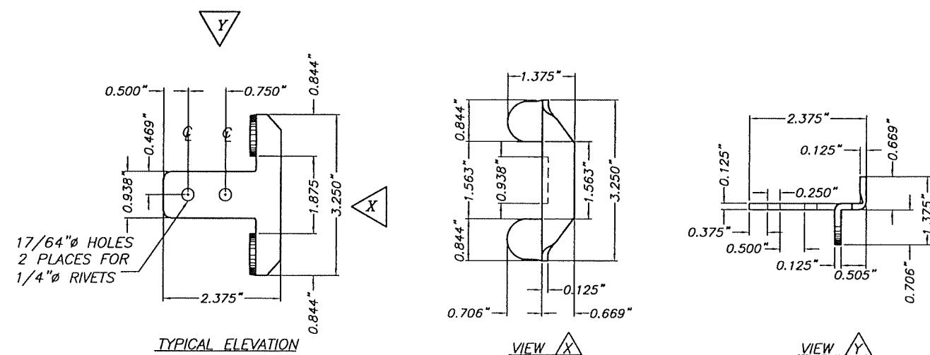
③ TYPICAL WINDLOCK W - 1 DETAIL SCALE : 3/8" = 1"
