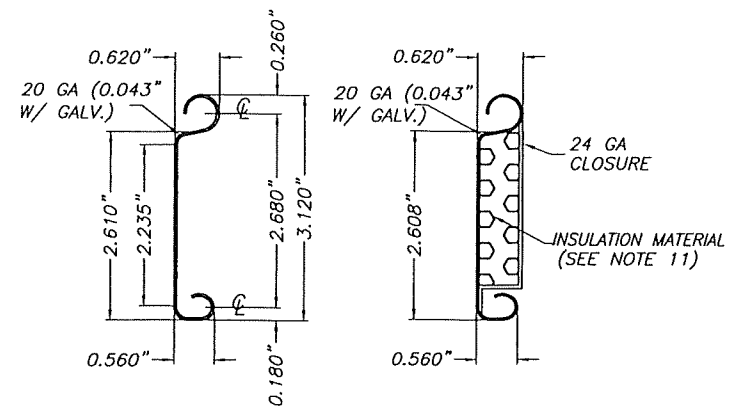
PLAIN INSULATED
