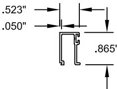
36 BEAD C #7042, 6063-T6
