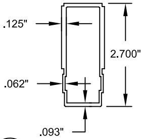
71 FRAME ASSEMBLY TUBE #7004, 6063-T6
