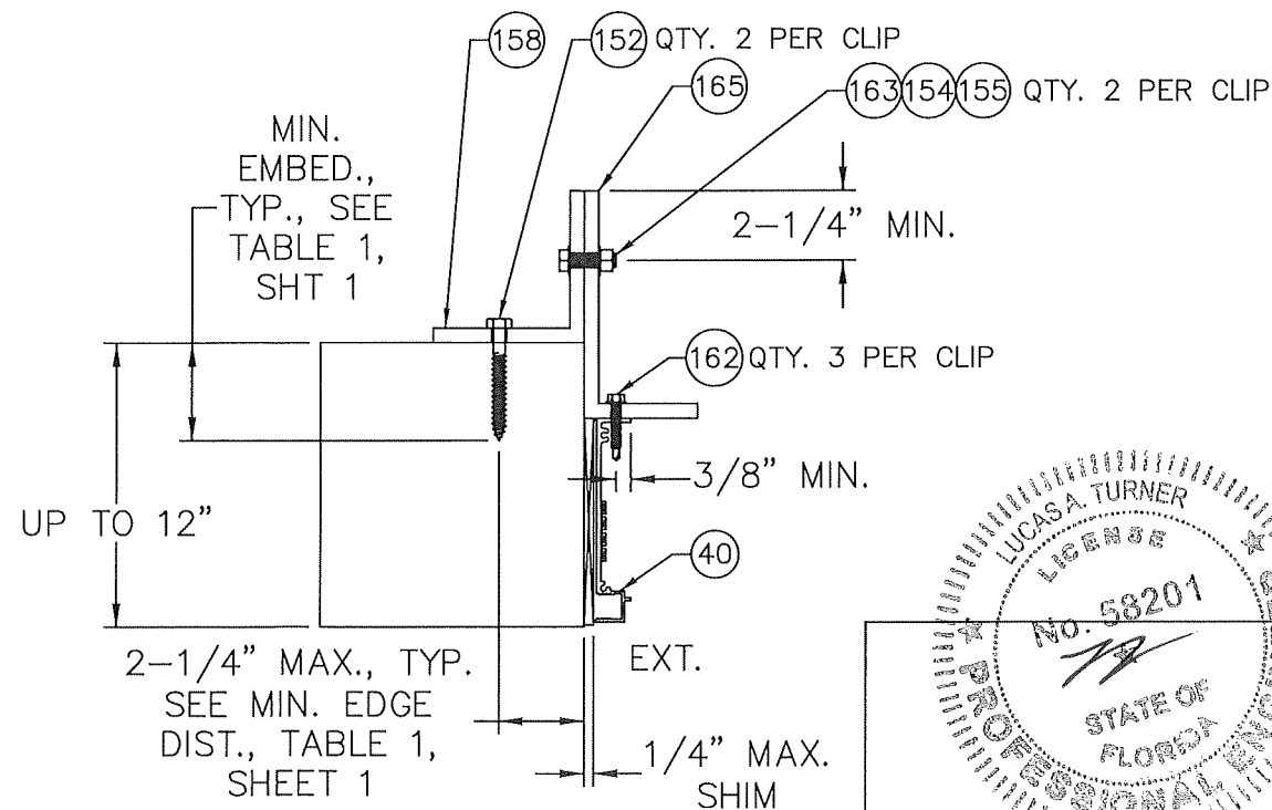
C 3x3x3/8" ALUMINUM JAMB CLIP OPTIONAL ATTACHMENT TO UP TO 12" WALL WITH MOUNTING ANGLE
