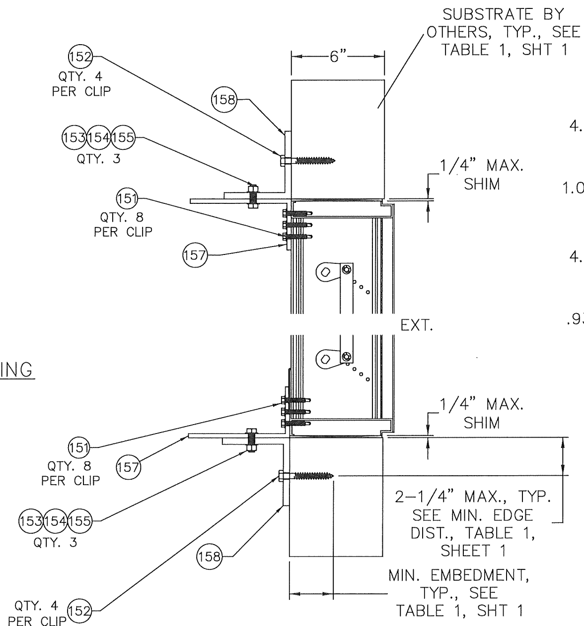
3x6x1/4" ALUMINUM MULL CLIP HEAD/SILL OPTIONAL ATTACHMENT TO 6" WALL WITH 4X4X3/8" ALUMINUM MOUNTING ANGLE
