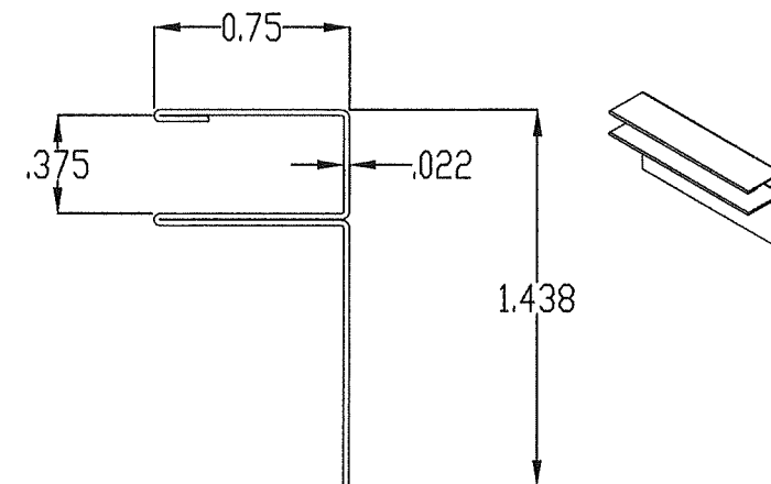
3 F-CHANNEL ALUMINUM 0.022" THICK
