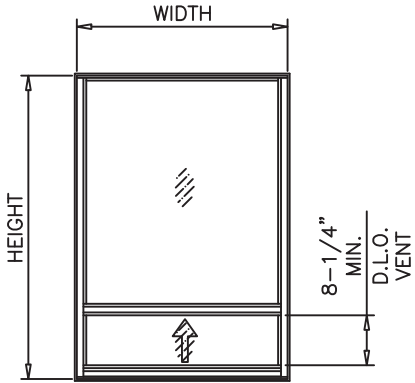
UNEQUAL LITE (ORIEL TYPE)
