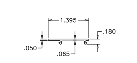
M3 FLUSH FRAME COVER
