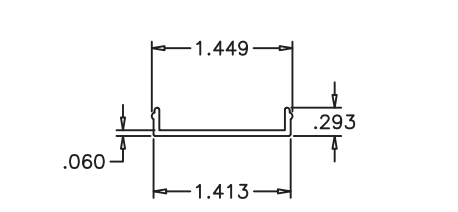
M19 SCREW COVER
