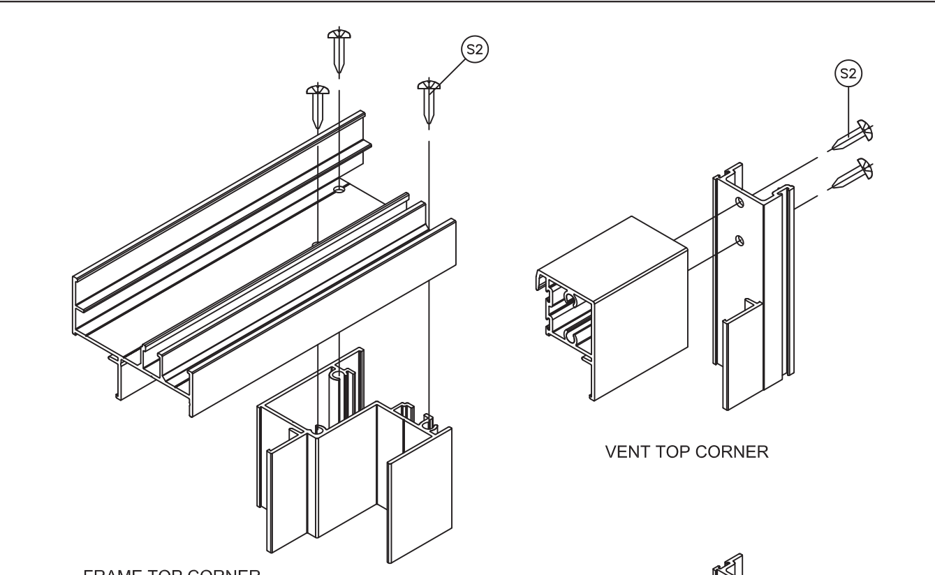
FRAME TOP CORNER
