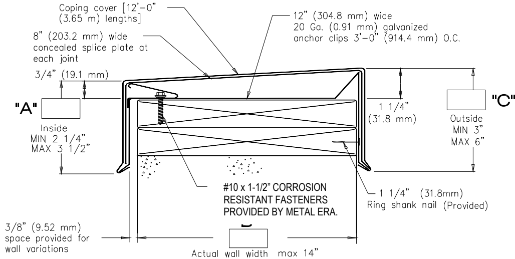
PERMA-TITE COPING (14" WIDE)
