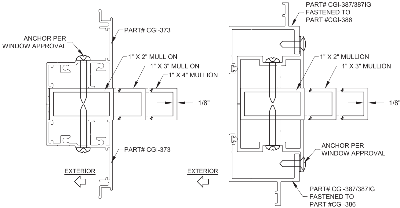
WINDOW-TO-MULLION DETAIL
