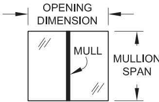
POINT LOADED MULLION (SEE NOTE 5 )
