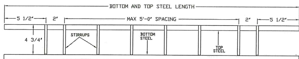
LINTEL REINFORCING CAGE FABRICATION MODEL
