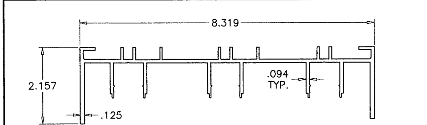
E19 FRAME HEAD (WITHOUT HEAD RECEPTOR)
