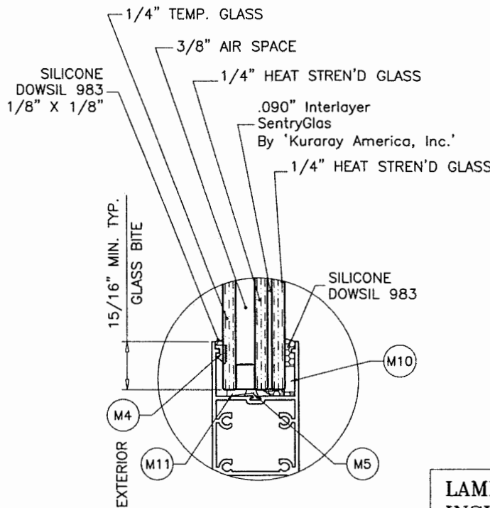
GLASS TYPE 'BI'
