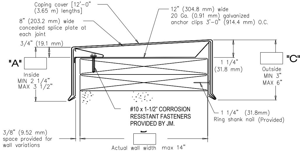
PRESTO-LOCK COPING (14" WIDE)
