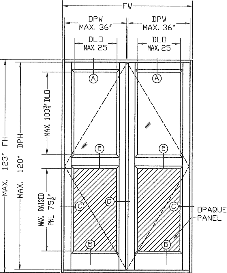
TYPE 5 SPLIT PANEL CONFIGURATION
