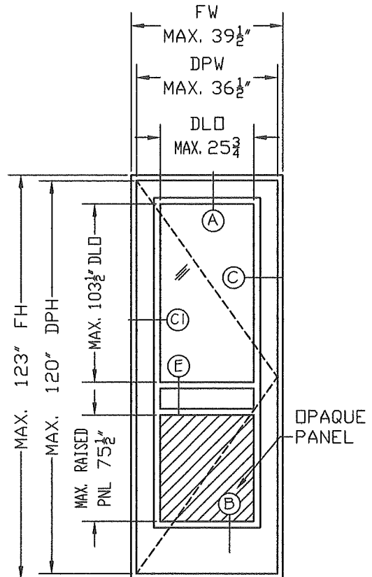
TYPE 4 LITE WITH PANEL CONFIGURATION
