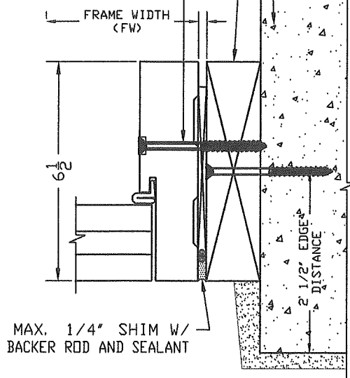
OPTION 3 FRAME WITH MAXIMUM 1/4" PT WOOD SHIM AND SECURED TO THE 2X PT CONT. WOOD BUCK WITH #14 SS WOOD SCREWS OR 1/4" ULTRACONS WITH 1 1/2" MIN. EMBEDMENT INTO WOOD (SG=.55) (SEE SHEET 3 FOR ANCHORS LAY-OUT)
