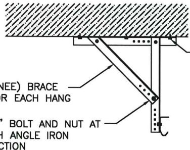
HANG DETAIL A-A HANGS CAN BE MOVED TO MATCH CEILING STRUCTURE
