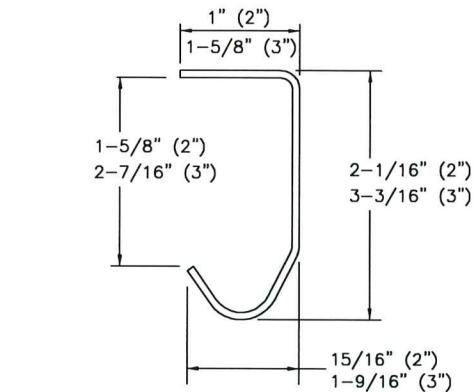
TRACK (2" AND 3") 0.075" OR 0.083" GALV. STEEL (2") 0.101" GALV. STEEL (3")
