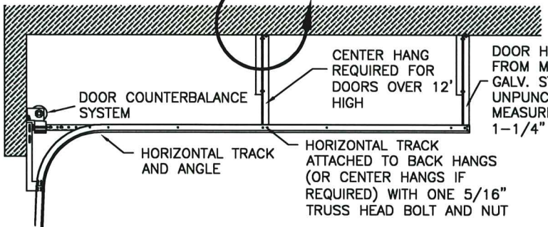
HORIZONTAL TRACK STANDARD LIFT TRACK SHOWN. LOW HEADROOM, HIGH LIFT AND VERTICAL LIFT TRACK ALSO AVAILABLE.
