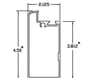
END STILE, BOTTOM & TOP RAIL 105008 - .075" WALL * DOORS WITH 1" JAMB OVERLAP THESE END STILE DIMENSIONS ARE 1" LONGER (5.50 & 4.812)
