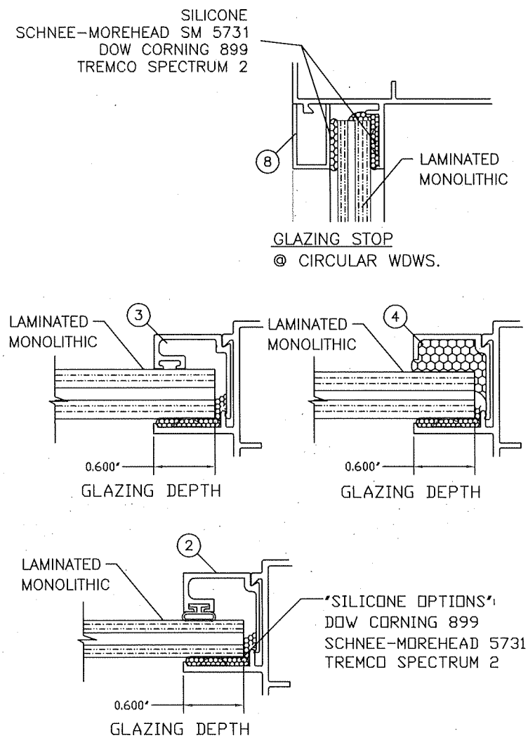
LAMINATED/MONOLITHIC GLASS TYPICAL GLAZING DETAIL
