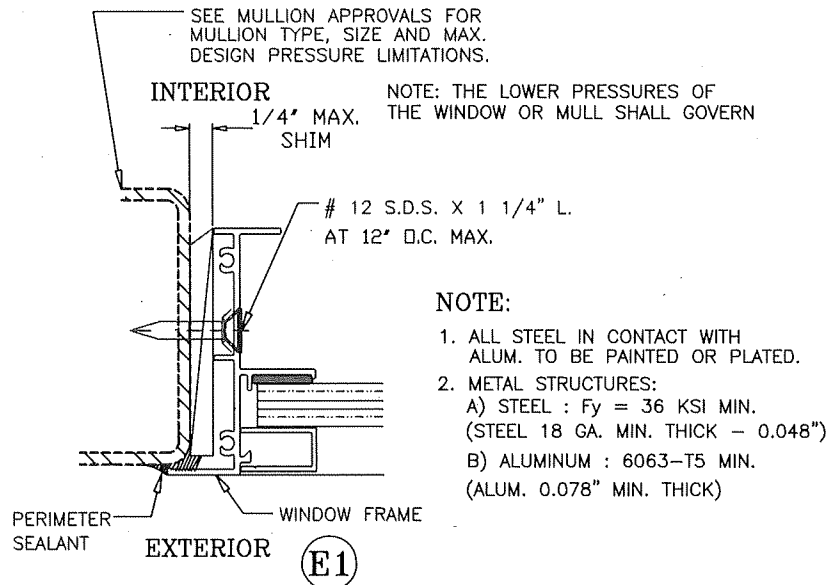
METAL STRUCTURE ATTACHMENT DETAIL
