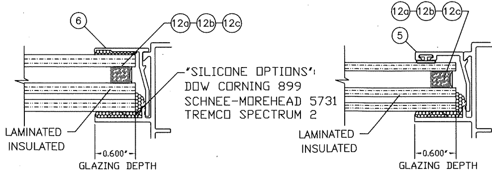
LAMINATED/INSULATED GLASS TYPICAL GLAZING DETAIL
