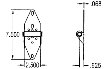
P/N 400735-XXXX, CENTER HINGE STANDARD (ATTACH WITH (4) 1/4"-14 X 7/8" SELF DRILLING CRIMPTITE SCREWS)
