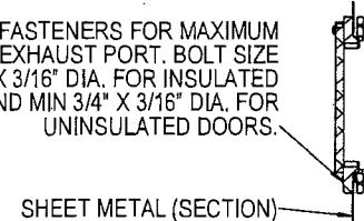
EXHAUST PORT DETAIL SECTION G-G SCALE 1:4
