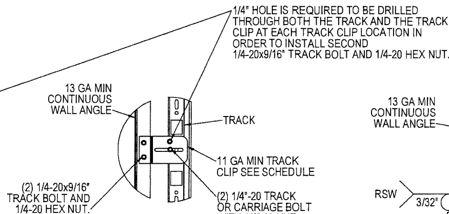
TYPICAL TRACK CLIP BOLTING DETAIL
