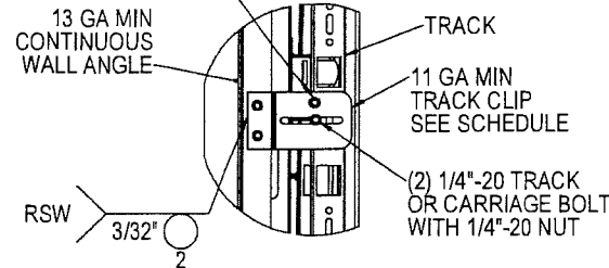
TYPICAL TRACK CLIP WELDING DETAIL
