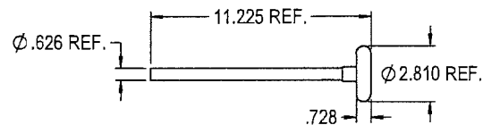
P/N 404046-0002, ROLLER ASSY. 3" TR-7 5/8" STEM
