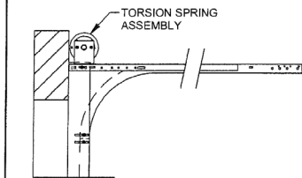
NORMAL HEADROOM TRACK 2" TRACK ANGLE MOUNT SHOWN 3" TRACK ANGLE MOUNT AVAILABLE
