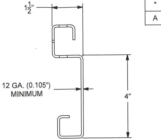
13 SLAT DETAIL TYPICAL SECTION SEE NOTE 6.1 FOR MATERIAL SPECIFICATIONS SCALE 3/8
