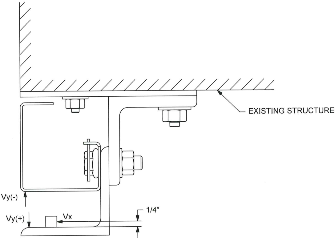
⑪ SUPERIMPOSED LOAD DIAGRAM - Z GUIDE SCALE 3/8
