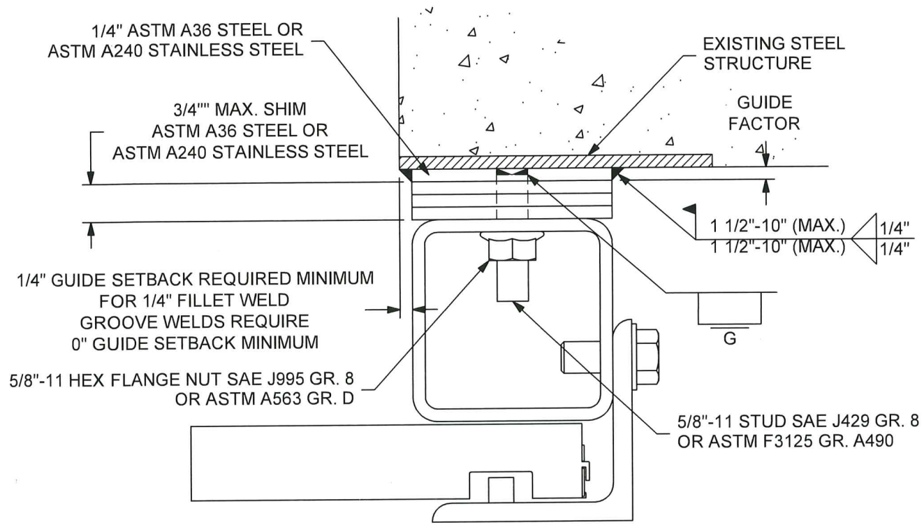
8 GUIDE ASSEMBLY - BOX GUIDE TO STEEL STRUCTURE WITH STUD PLATE SCALE 3/8
