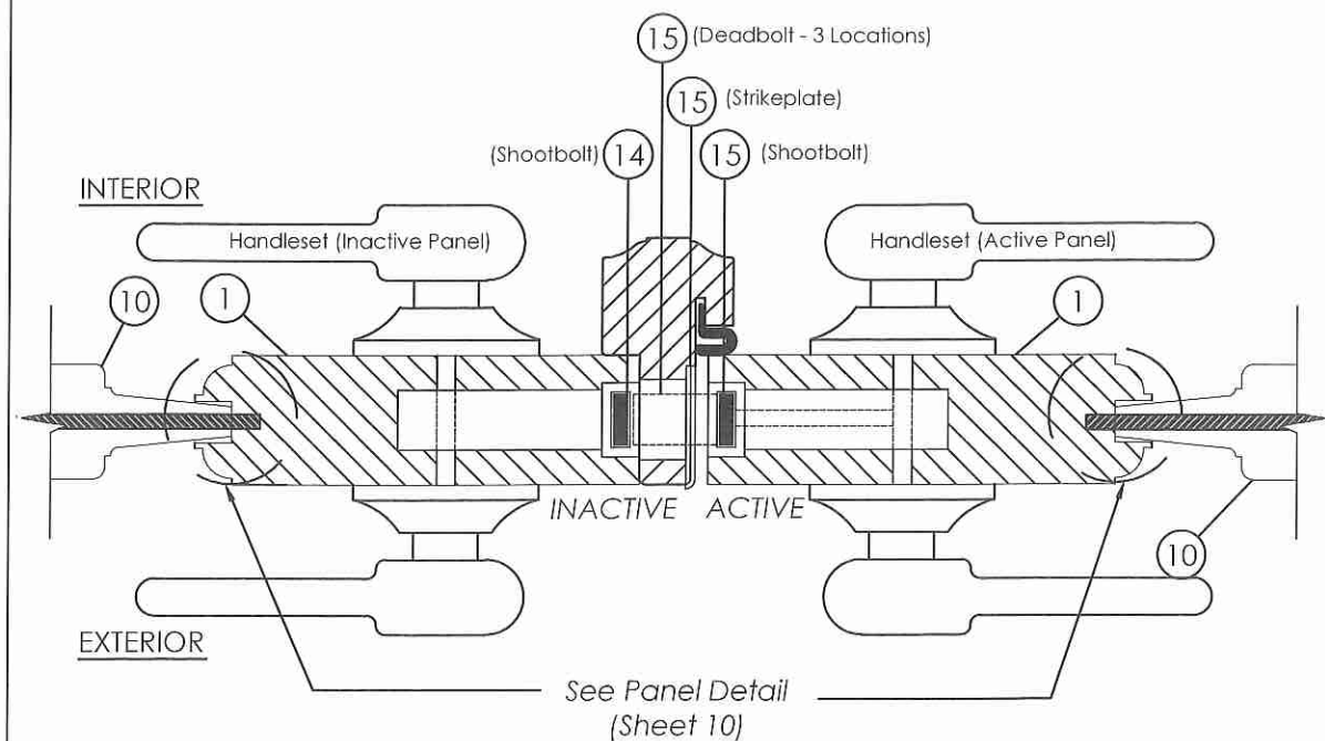
R 12 HORIZONTAL SECTION MULTI-POINT LOCK OPTION
