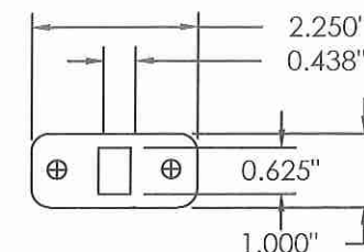
SHOOTBOLT STRIKE PLATE Face View
