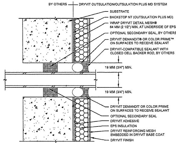
PENETRATIONS
