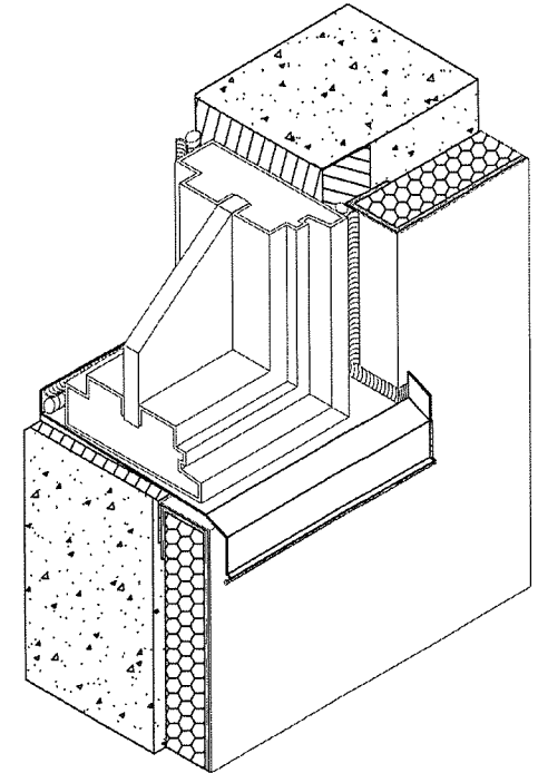
WINDOW OPENING
