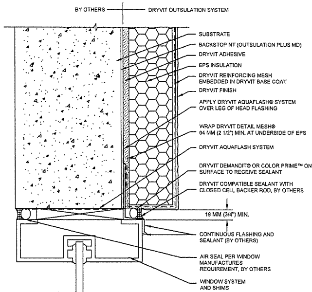
HEAD TERMINATION
