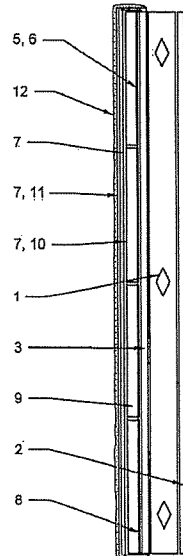
SECTION B-B
