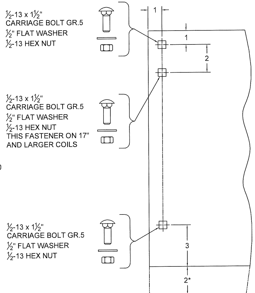
⑥ WINDLOCK DETAIL CAST MALLEABLE IRON ASTM A47, GRADE 32510, OR DUCTILE IRON PER ASTM A536 GRADE 65-45-12, GALVANIZED IN ACCORDANCE WITH ASTM A123, GRADE 85 ZINC-COATING 1/2 SCALE
