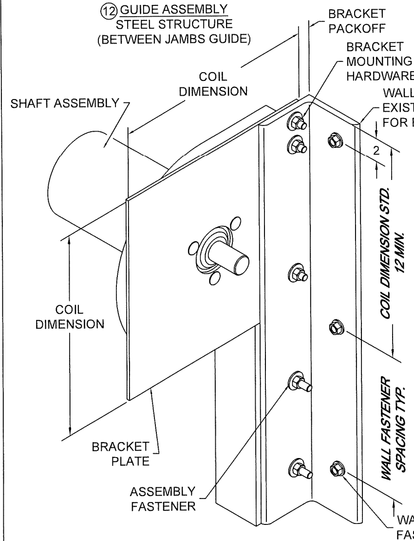
13 BRACKET MOUNTING / TOP WALL ANGLE FASTENING BRACKET MOUNTING PER DETAIL 7 DEPICTED, OTHER BRACKET MOUNTINGS ARE AVAILABLE SCALE: NTS
