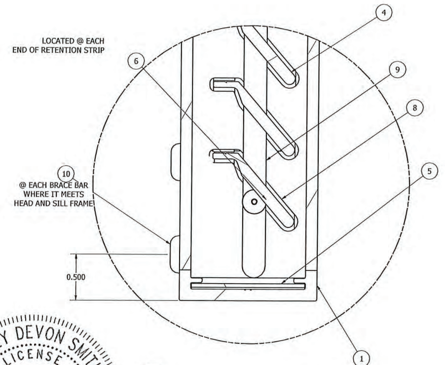
6 2 SILL CONSTRUCTION DETAIL N.T.S.
