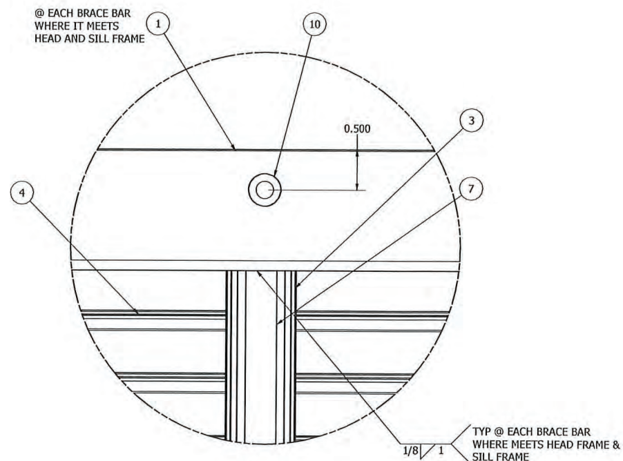
5 2 BRACE BAR WELDMENT CONSTRUCTION DETAIL N.T.S.
