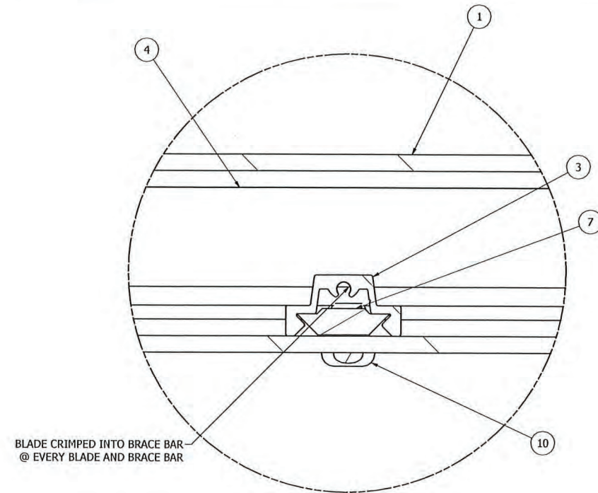
2 2 BRACE BAR CONSTRUCTION DETAIL N.T.S.
