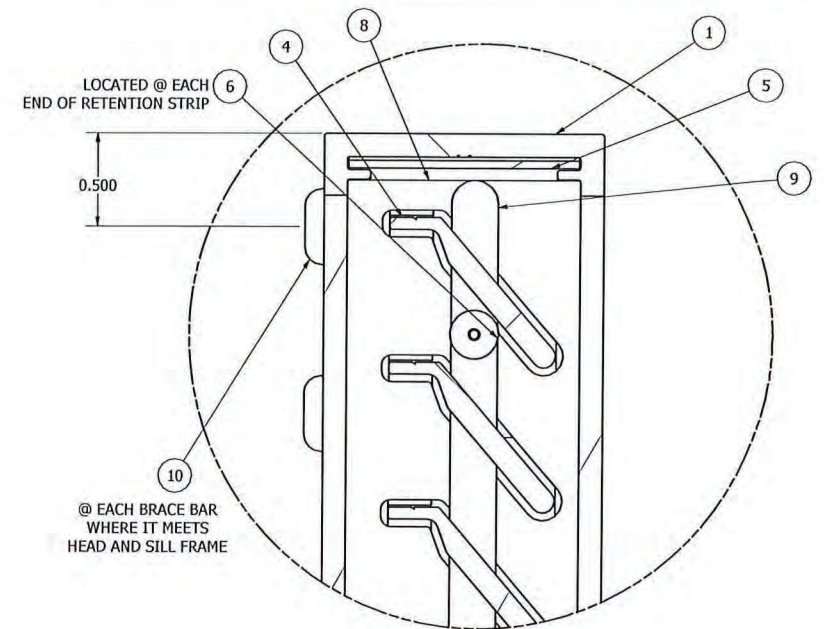
3 2 HEAD CONSTRUCTION DETAIL N.T.S.
