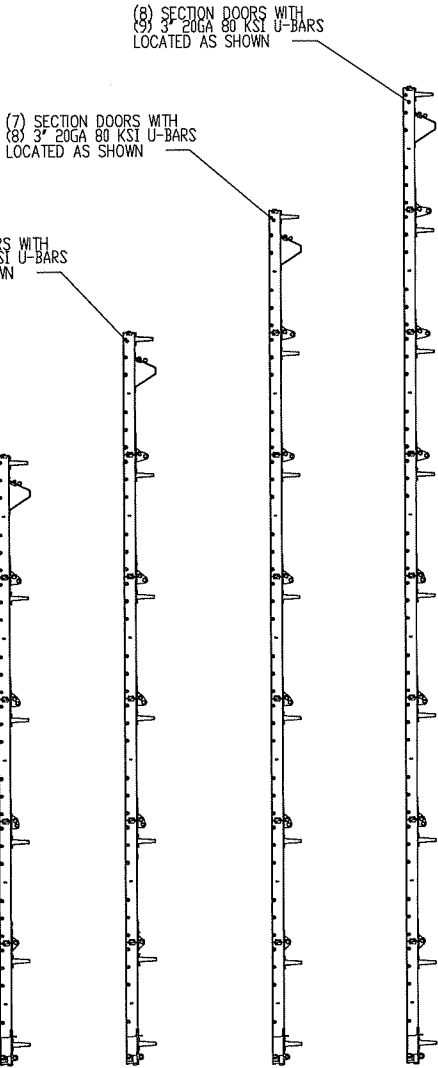
STRUT LOCATIONS SCALE 1 : 16
