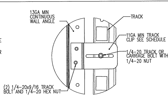
TYPICAL TRACK CLIP BOLTING DETAIL
